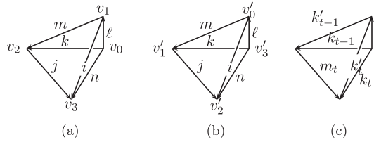
Fig. 9. A standard tetrahedron labeling and edge orientations (a), and two other labelings.
