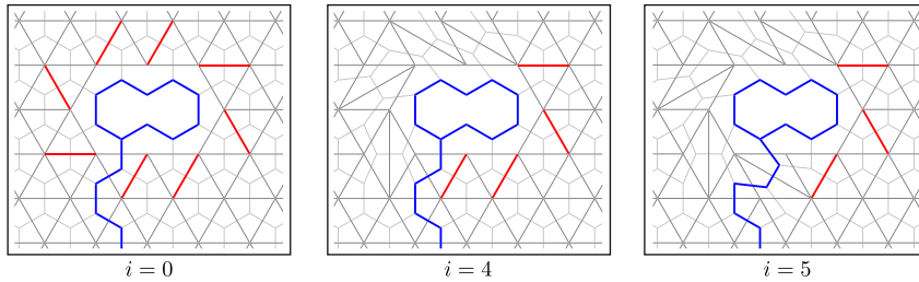
Fig. 7. This figure shows for various i how i F -moves in the first round ( r=1 ) of the Dehn-twist D(\gamma) affect a ribbon graph |\Phi\rangle \in \mathcal{H}_\Lambda^{(\ell,0^p)} embedded in the dual graph \hat{T} .
