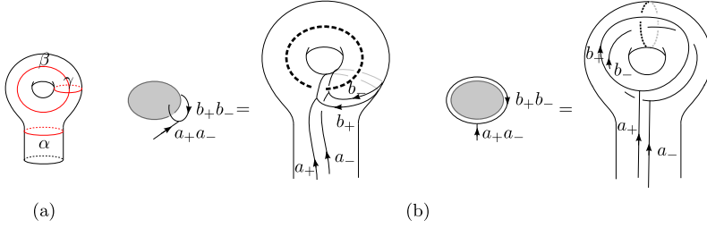
Fig. 12. An anyonic fusion basis for a surface with n punctures or handles is specified by using for each handle one of the two bases in (b), combined with a doubled anyon fusion tree in \Sigma_n \times [-1, 1] .
