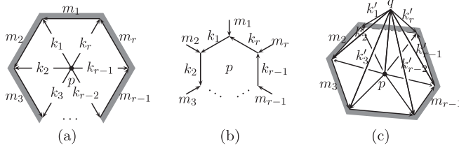
Fig. 10. The neighborhood of a vertex p in a triangulated surface can be oriented as in (a), in turn orienting the trivalent dual graph in (b). Attaching a “blister” above p gives (c) when r = 6 .
