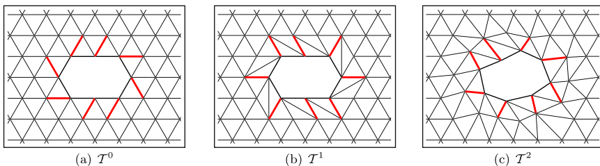
Fig. 6. From left-to-right, the triangulations T^0 , T^1 and T^2 obtained while implementing a Dehn-twist about the inner curve \gamma . The portion \Sigma_L of the surface within \gamma is not shown. The thick, red edges are the locations of F -moves in the next round, i.e., the edges \{e_i\} . (For interpretation of the references in colour in this figure legend, the reader is referred to the web version of this article.)
