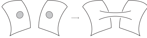
Fig. 15. Two surfaces can be joined by puncturing each and identifying the boundaries of the holes, as in Section 5.1. In the case that the surfaces are the same, the boundary of a 3-manifold, gluing together two disks from the boundary adds a handle to the manifold. The Turaev–Viro state for the resulting manifold has a vacuum loop going around the handle.
