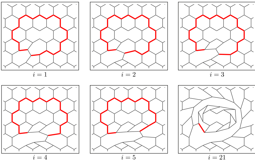
Fig. 5. The successive figures show the intermediate steps of the \text{cut}(\gamma) procedure, after applying F_{e_i} . The thick, red edges are e_1, \dots, e_n . The overall effect of the procedure is shown in Fig. 4. (For interpretation of the references in colour in this figure legend, the reader is referred to the web version of this article.)
