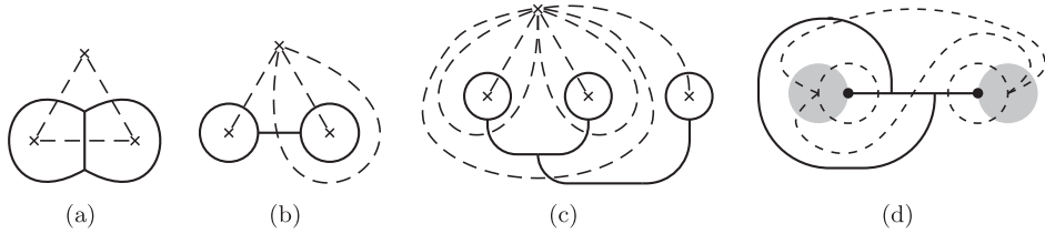
Fig. 1. In (a) and (b) are shown two different examples of basis choices for \mathcal{H}_\Sigma for the case of \Sigma being the sphere with three punctures (indicated with crosses). Dashed lines mark the point-set triangulation of the punctures, while the dual graph, which is trivalent, is indicated with solid lines. Part (c) gives another example of a basis for the sphere with four punctures. In (a)–(c), it is assumed that there are no marked points on the boundaries of \Sigma . Part (d) shows the more general situation, for the sphere with two shaded holes, each of which has a marked point on its boundary.
