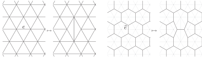
Fig. 3. Change of triangulation \mathcal{T} by flipping edge e (left), and the effect on the dual lattice \hat{\mathcal{T}} .
