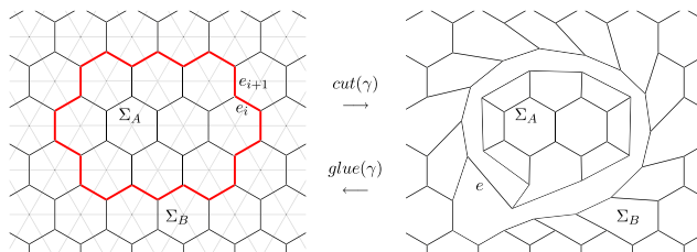
Fig. 4. The procedure cut(\gamma) isolates a region \Sigma_A enclosed by a closed curve \gamma , by making F -moves in sequence along the edges e_1, e_2, \dots, e_n , colored red, counterclockwise along \gamma on the dual graph \tilde{T} . The result is a tadpole-like structure as in Lemma 4.2, with a single edge e and plaquette q between the two regions. The inverse operation is glue(\gamma) . (For interpretation of the references in colour in this figure legend, the reader is referred to the web version of this article.)
