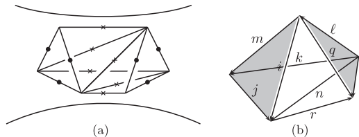
Fig. 16. Two triangulations of a handle, used in the proof of Lemma C.1.
