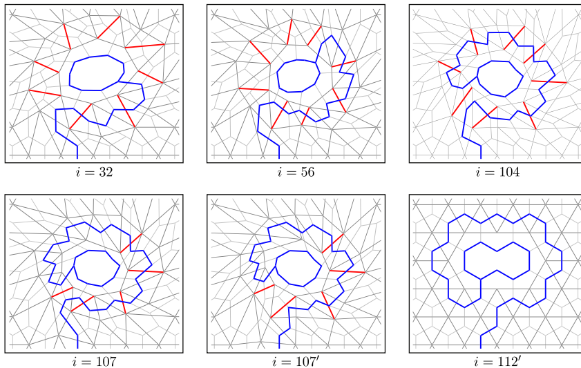
Fig. 8. This figure continues Fig. 7 for larger i , in order to illustrate that D(\gamma) indeed corresponds to the deformation of an off-lattice ribbon graph by a Dehn-twist. The half-Dehn-twist \sqrt{D}(\gamma) is implemented by i=56 F -moves. After the 107-th F -move, we switch from |\Phi\rangle \in \mathcal{H}_\Lambda^{(\ell,0^p)} to a different representative |\Phi'\rangle \in \mathcal{H}_\Lambda^{(\ell,0^p)} for convenience (note that B|\Phi\rangle = B|\Phi'\rangle ).
