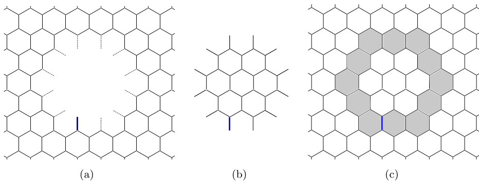
Fig. 2. The Levin–Wen model with a boundary, realizing \mathcal{H}_\Sigma^\ell : qubits sit on the solid lattice edges. In (a) and (b), dashed edges represent “virtual” qubits fixed to 0. The thick, blue edge represents a virtual qubit fixed to the label \ell(p) of the marked boundary point p . In (c) is illustrated the gluing of anyon fusion basis states described in Section 4.2. The t virtual qubits are replaced by qubits, and prepared in states |k\rangle \otimes |0\rangle^{\otimes (t-1)} , for k \in \{0, 1\} , entangled with states on either side. Subsequently, all plaquette operators touching the boundary (shaded plaquettes) are applied. (For interpretation of the references in colour in this figure legend, the reader is referred to the web version of this article.)
