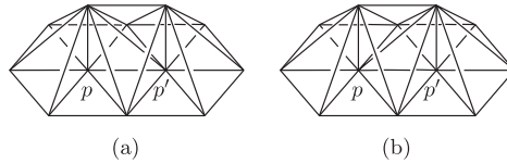
Fig. 11. For two adjacent vertices p and p' , the products B_{p'}B_p and B_pB_{p'} correspond to different internal triangulations of the same bipyramid. Hence B_p and B_{p'} commute.
