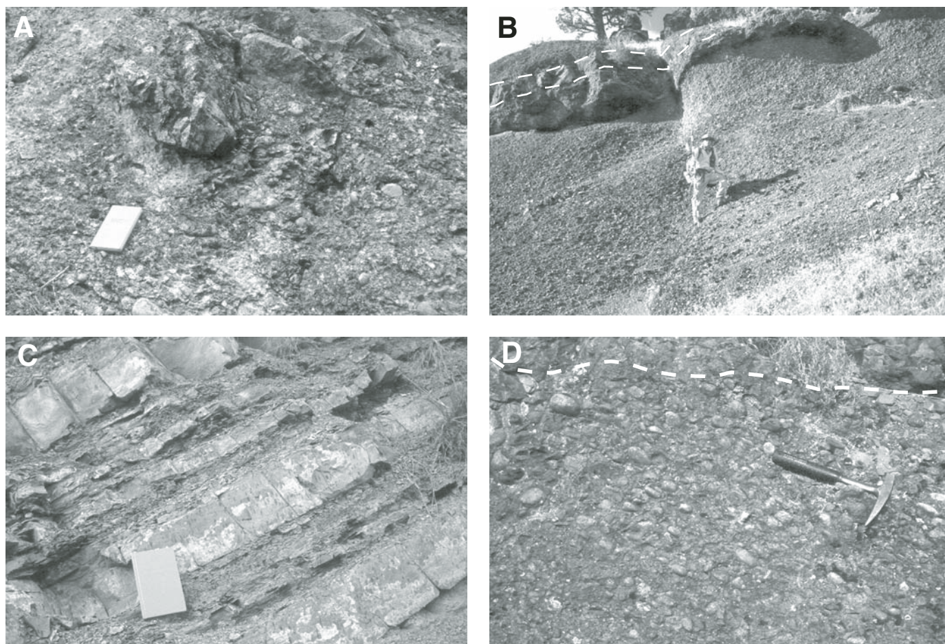
Figure 5. Outcrop photographs showing lithologies and features of Cretaceous strata in the Toney Butte area. (A) Clast-supported conglomerate of the basal Hudspeth Formation with oversized clasts of basement rock (upper part of photo). The largest clast, visible above the notebook, is ~80 × 20 cm. Notebook is 19 cm long. (B) Clast-supported conglomerate of the Gable Creek Formation showing very thick, massive nature and interbedded sandstone (dashed lines). Bedding dips obliquely away from viewer. (C) Bedded sandstone of the Gable Creek Formation, showing high sandstone:shale ratio typical of sand-rich turbidites. Notebook is 19 cm long. (D) Imbricated clast fabric in Gable Creek conglomerate. Dashed line indicates bedding (interbedded sandstone unit). Clasts dip to the right side of the photo indicating transport to the left. Hammer is 33 cm long.
