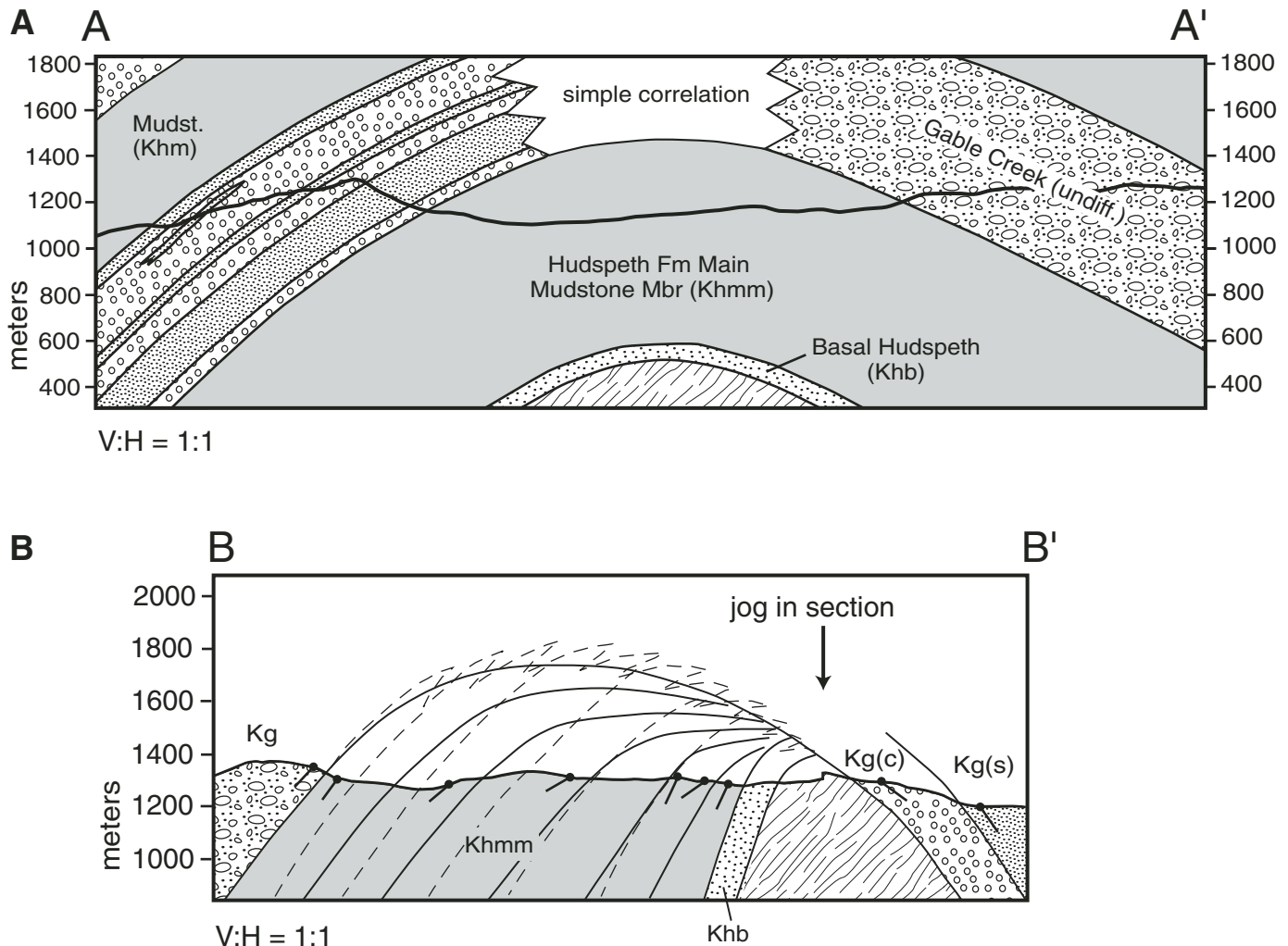
Figure 7. Geologic cross sections of the Toney Butte area. (A) Cross section A–A' (NW to SE) across the Mitchell anticline. (B) Cross section B–B' (N–S) across the Toney Butte anticline, showing two possible interpretations for the northward pinch-out of Main Mudstone member (Khmm) across basement-cored anticline. Solid lines represent wedging beds and progressive unconformity produced by growth of E-trending monocline during deposition of Khmm; dashed lines represent large lateral facies change from Gable Creek conglomerate in the north to Khmm mudstone in the south, and involves no syndepositional tilting. Solid-line interpretation is preferred, as discussed in text. Patterns are same as in Figure 2B; see Figure 2B for location of section lines. Kg—Gable Creek (undifferentiated); Kg(c)—Gable Creek Formation conglomerate; Kg(s)—Gable Creek Formation sandstone; Khmm—the Main Mudstone member of the Hudspeth Formation.
