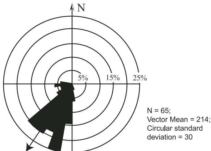
Figure 6. Rose diagram of paleocurrent data from clast imbrications in the Gable Creek Formation, restored to horizontal using bedding strike and dip, present-day coordinates. After restoring for \sim 37^\circ of post-Albian clockwise rotation (Housen and Dorsey, 2005), southwest-directed paleocurrents restore to south-directed for middle Cretaceous time.
