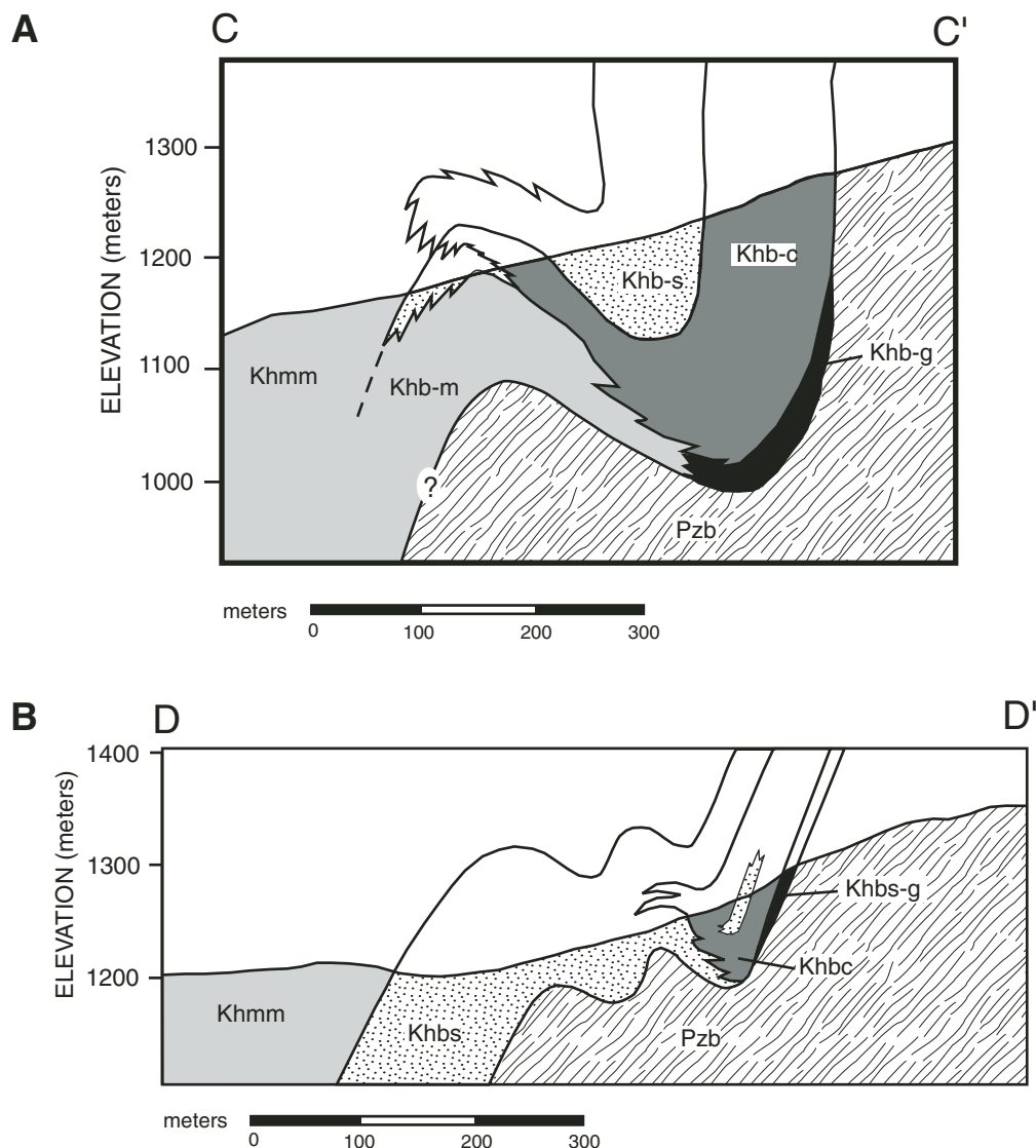
Figure 9. Detailed geologic cross sections. (A) Cross section C–C' on the southwest flank of Toney Butte. (B) Cross section D–D' on the south flank of Toney Butte. Both cross sections show tight, asymmetric folds and rapid lateral facies changes from coarse-grained basal Hudspeth units into mudstone. Subunits of basal Hudspeth Formation: Khbs-g—green sandstone; Khbm—mudstone; Khbc—conglomerate; Khbs—tan sandstone. Khmm—Main Mudstone member of Hudspeth Formation; Pzb—Paleozoic basement rocks. Patterns are same as in Figure 2B; see Figures 2B and 8 for location of cross sections.
