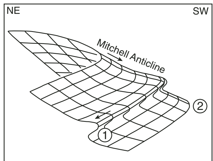
Figure 12. Schematic model for superposed folds at Toney Butte. Early folds (1) formed with ~NW trend (present coordinates) during deposition of the Main Mudstone member; this sketch illustrates a minor fold parasitic to the Toney Butte anticline. These were later folded about the Mitchell anticline axis (2) and rotated into their present orientations during Tertiary deformation.
