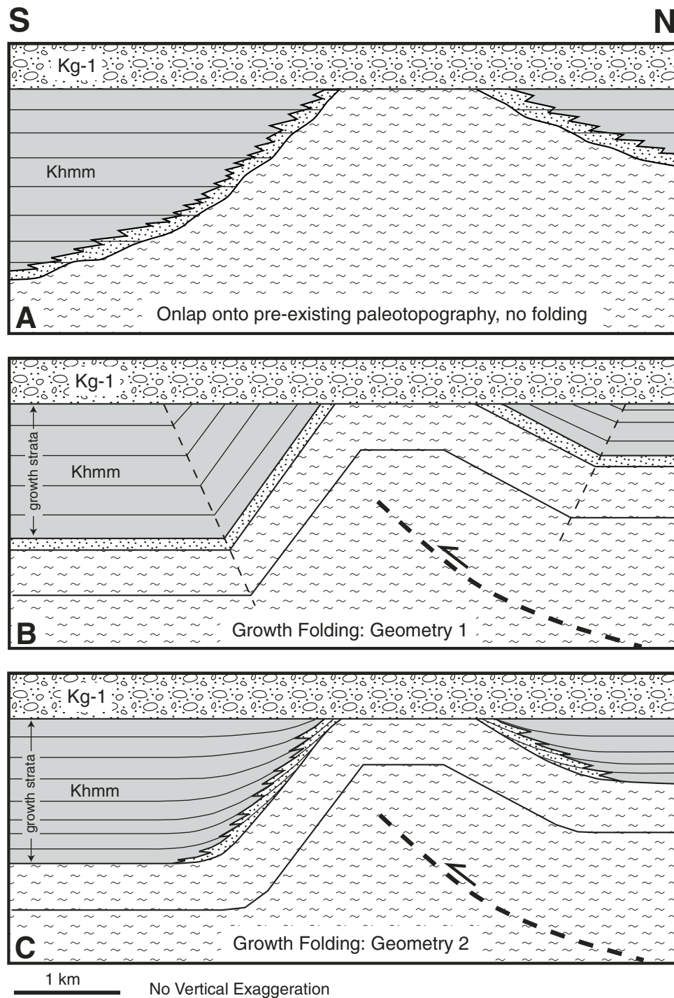
Figure 11. Three hypothetical models for the Toney Butte anticline based on restoration of cross section B–B' (Fig. 7B) to its pre–Gable Creek orientation. This also restores \sim 37^\circ of post–Gable Creek clockwise rotation (Housen and Dorsey, 2005). (A) Traditional hypothesis for pinch-out of the Hudspeth Main Mudstone member (Khmm) by stratigraphic onlap onto preexisting erosional topography, with no syn-Hudspeth folding. (B) Growth-fold hypothesis assuming fold geometry 1 (e.g., Suppe and Medwedeff, 1990; Suppe et al., 1992). (C) Growth-fold hypothesis assuming fold geometry 2 (e.g., Hardy and Poblet, 1994; Patton, 2004). We conclude that the growth-fold hypothesis in C is most consistent with the field data and observations. See text for discussion.
