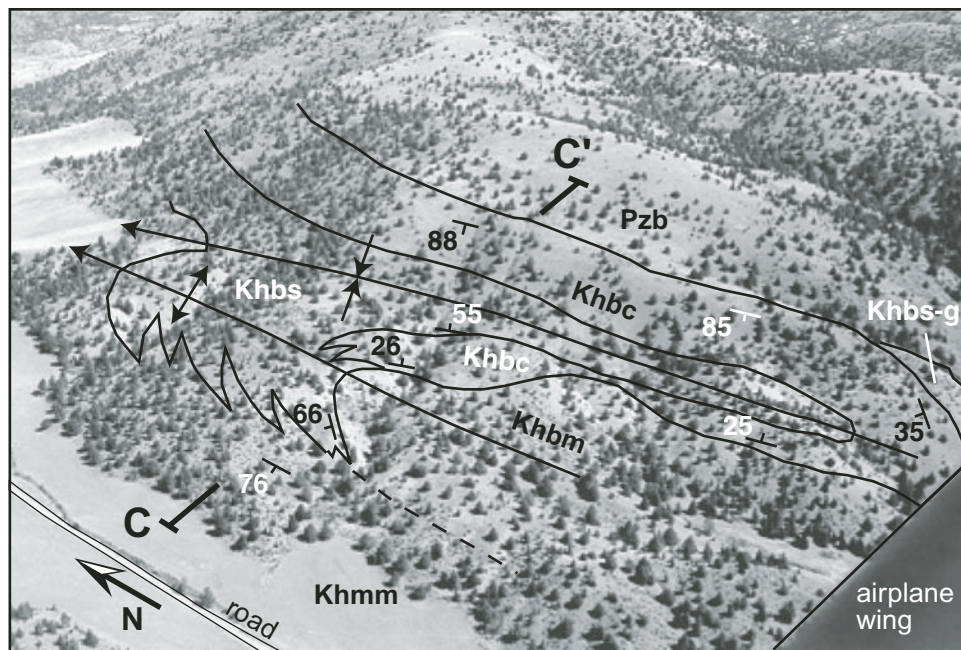
Figure 8. Oblique aerial photograph with contact lines based on 1:6000-scale mapping, showing tight folds in basal member of Hudspeth Formation on the southwest flank of Toney Butte. Sub-units of basal Hudspeth Formation: Khbs-g—green sandstone; Khbm—mudstone; Khbc—conglomerate; Khbs—tan sandstone (Fig. 3). Khmm—Main Mudstone member of Hudspeth Formation; Pzb—Paleozoic basement rocks. Location of this area indicated by position of cross section C–C' in Figure 2B. Line of section is ~700 m long.
