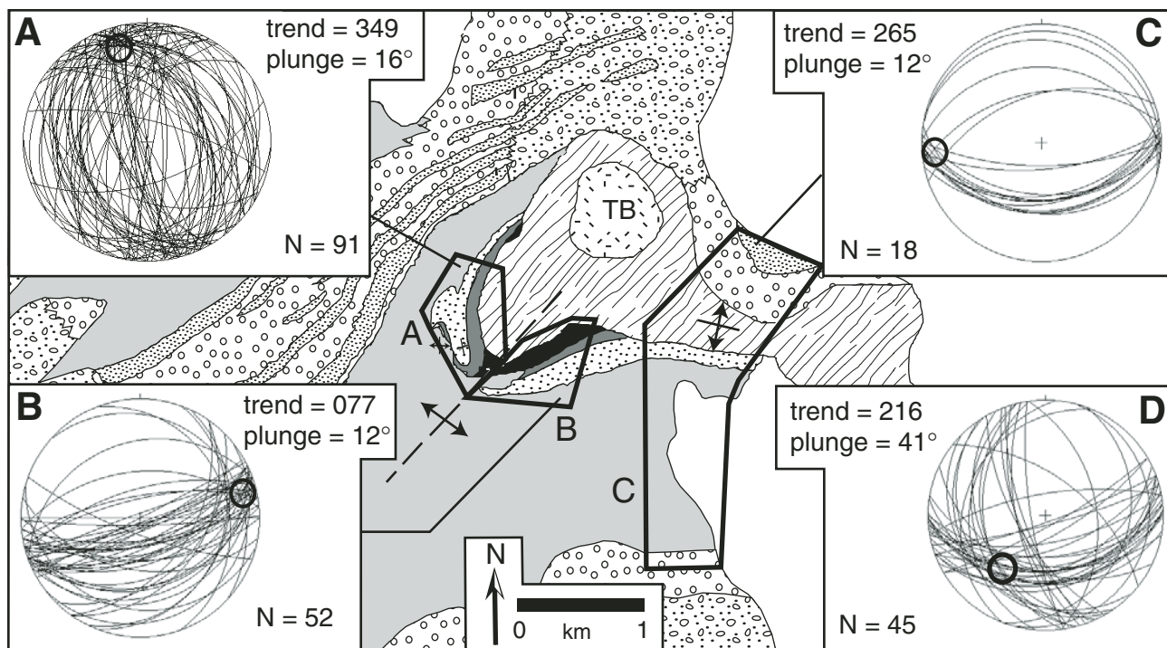
Figure 10. Simplified geologic map of the Toney Butte field area showing structural domains A to C, and stereonets with results generated by fold analysis. Domain D (not shown on map) is a small area in the immediate vicinity of the Mitchell anticline axis. See text for explanation. TB—Toney Butte.
