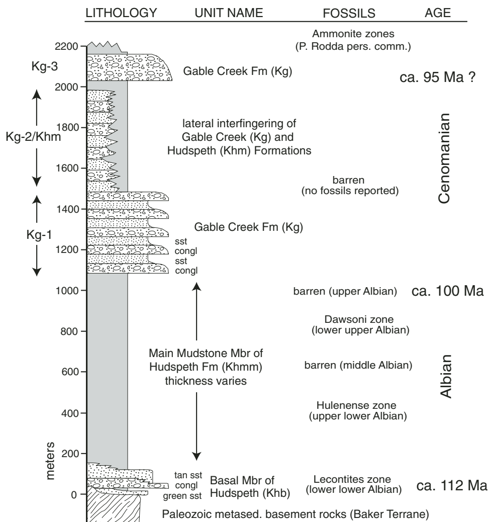
Figure 3. Composite stratigraphic section for the Toney Butte area. Patterns same as in Figure 2B.
