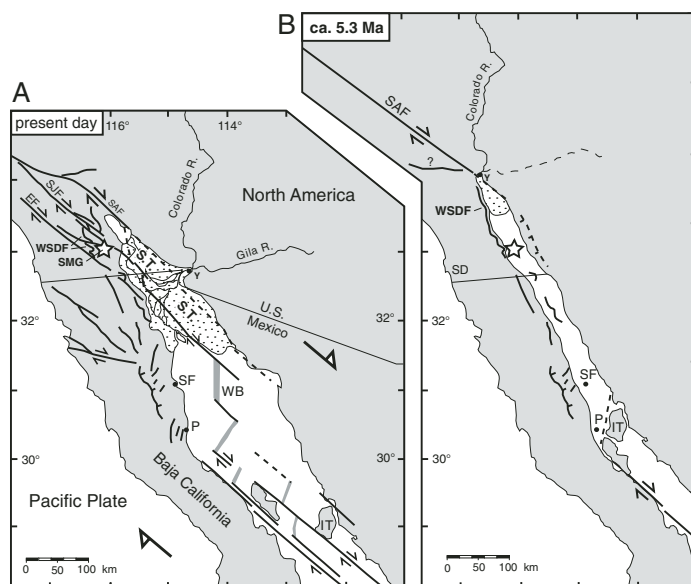
Figure 1. A: Regional tectonic map showing major faults in southwestern California and northwestern Mexico, and location of Split Mountain Gorge (SMG, star) in western Salton Trough. B: Reconstruction for 5.3 Ma restores ca. 250 km of dextral offset based on data of Oskin and Stock (2003b). EF—Elsinore fault, IT—Isla Tiburón, P—Puertecitos, SAF—San Andreas fault, SF—San Felipe, SJF—San Jacinto fault, S.T.—Salton Trough, WB—Wagner basin, WSDF—West Salton detachment fault, Y—Yuma. Stipple pattern shows area of subaerial Colorado Delta deposition, observed in the modern setting and inferred for 5.3 Ma.
