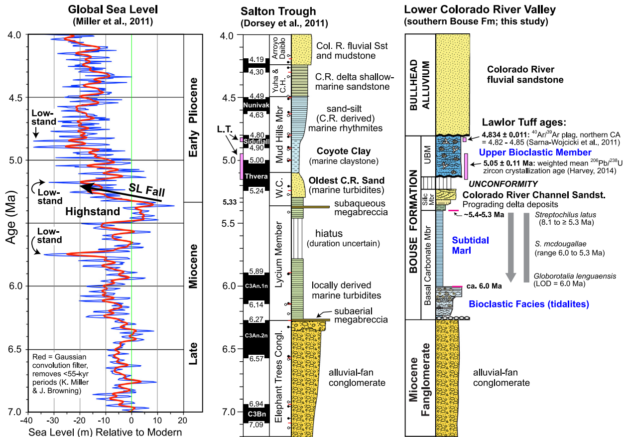
Fig. 21. Comparison of chronostratigraphy from 7 to 4 Ma in the Salton Trough and lower Colorado River valley to the global eustatic sea-level curve (Miller et al., 2011). The comparison provides powerful insights into controls on base-level change and sediment discharge during initiation and early evolution of the Colorado River. See text for discussion.
