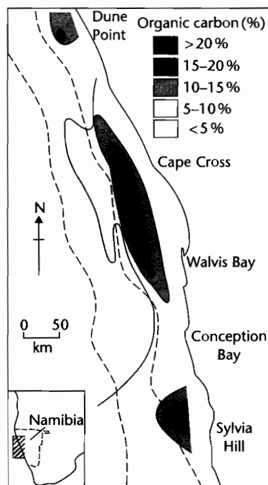
Fig. 10.15 Upwelling zone, offshore Namibia, showing oxygen-depleted zone, and total organic carbon concentrations of up to 26% (after Demaision and Moore 1980). Upwelling causes high phytoplankton productivity in surface waters. The sea bottom sediments are anoxic under the highly productive waters.
