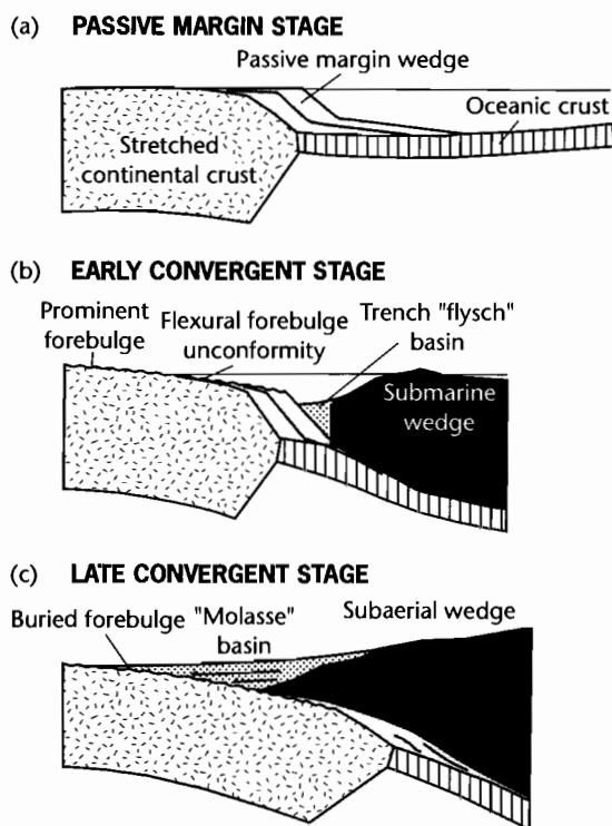
Fig. 4.31 Model involving orogenic loading of a previously stretched continental margin during the early stages of convergence (Stockmal et al. 1986; Watts 1992), modified by Allen et al. (1991). The first orogenic loads are emplaced on a weaker lithosphere at considerable water depths.
