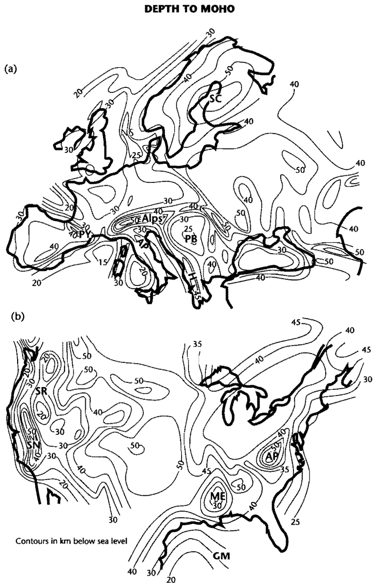
Fig. 1.2 Depth to the Moho below sea-level from (a) Europe and (b) North America, after Allenby and Schnetzler (1983) and Meissner (1986). In Europe, thick continental crust occurs in the Pyrenean–Alpine–Carpathian orogenic belt and in the Scandinavian Shield. Thin continental crust occurs along the Atlantic margin and in regions of continental stretching, such as the North Sea, western Mediterranean, Pannonian Basin, and Black Sea. In North America, thick continental crust is associated with the batholiths of the Sierra Nevada region, the Appalachian orogenic belt, the American midcontinent and the Canadian–NE USA shield. Thin crust is associated with the plateau basalts of the Snake River area, sites of rifting such as the Mississippi Embayment, and along the western active continental margin, eastern passive continental margin and the Gulf of Mexico. NS, North Sea; SC, Scandinavian Shield; PY, Pyrenees; AP, Apennines; PB, Pannonian Basin; H, Hellenides; SR, Snake River; SN, Sierra Nevada; ME, Mississippi Embayment; AP, Appalachians; GM, Gulf of Mexico. Reproduced courtesy of Elsevier.
