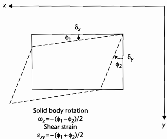
Fig. 2.4 Deformation of a rectangle into a parallelogram by a strain field involving shear.
