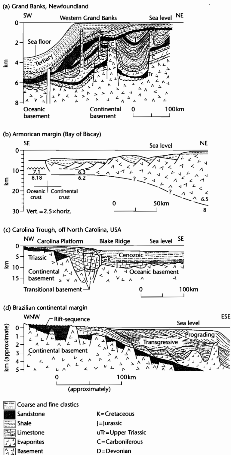
Fig. 8.54 Types of passive margin stratigraphy around the Atlantic Ocean. (a) The sediment-nourished margin of Grand Banks, Newfoundland shows complex unconformities and salt diapirism originating from the Jurassic; (b) The sediment-starved Armorican margin (Bay of Biscay) retains deep water depths; (c) Carolina Trough, eastern US seaboard has a thick Jurassic carbonate bank extending onto oceanic basement; (d) Brazilian continental margin shows salt diapirism originating in the Lower Cretaceous and prograding clastic wedges. Modified after Miall (1984).
