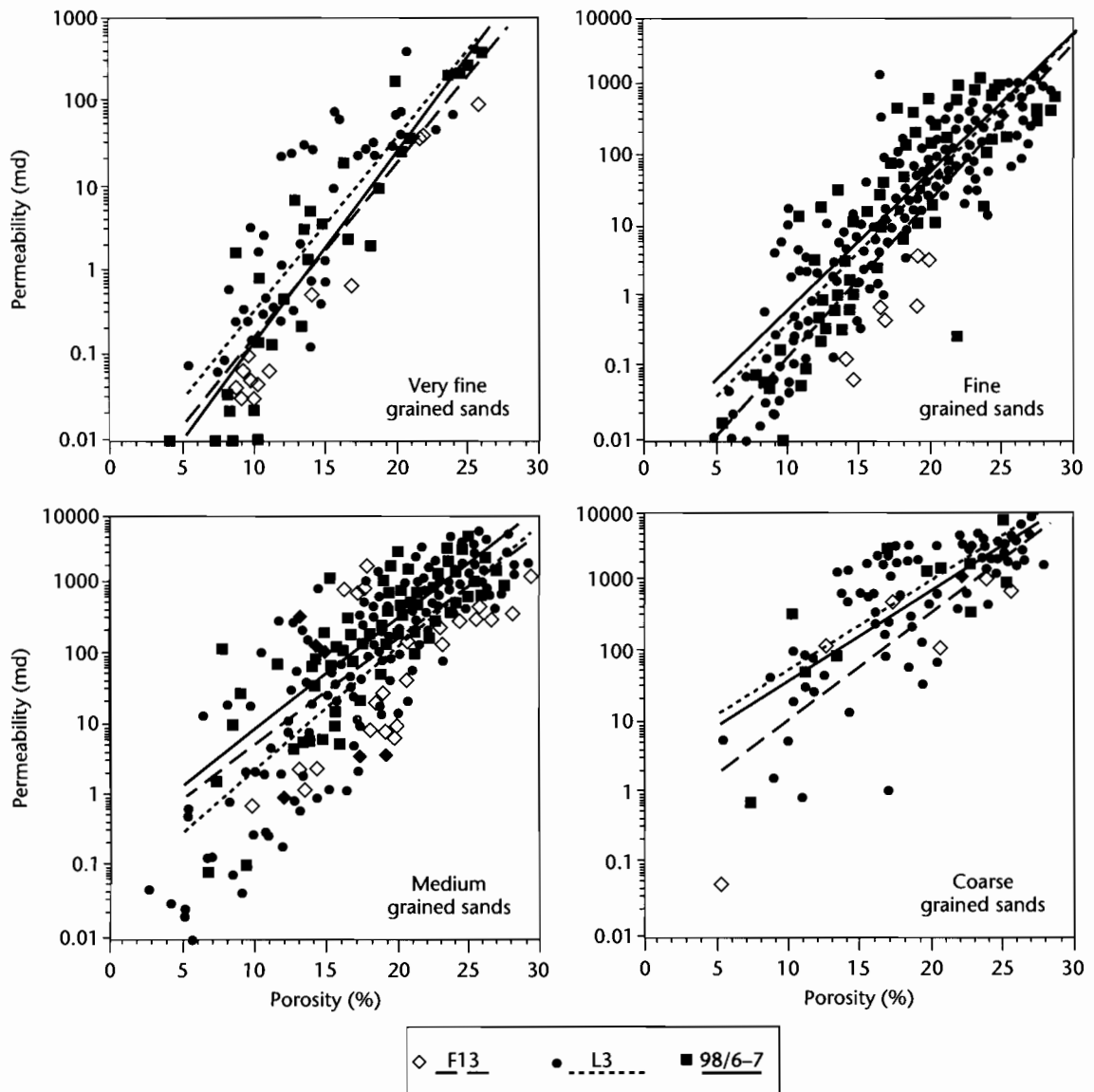
Fig. 10.40 Relationship of permeability with horizontal core plug porosity for four grain size classes in the Triassic Sherwood Sandstone reservoir in three wells in the Wytch Farm field, Dorset, UK. After Hogg et al. (1996). Reproduced courtesy of Geological Society of London.
