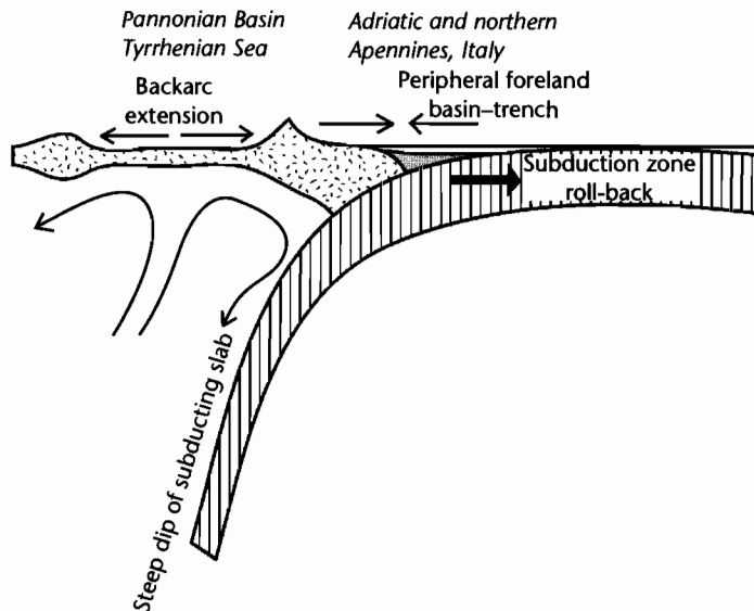
Fig. 4.1 Schematic illustration of peripheral foreland basins, retro-foreland basins, and basins related to subduction zone roll-back.
