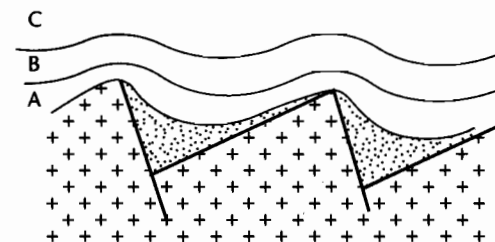
Fig. 10.60 Formation of drape anticline by differential compaction. Relief of anticline increases with depth. Basement topography causes thickness variations in the compactible sediment column. As these sediments compact, drape anticlines are formed.
