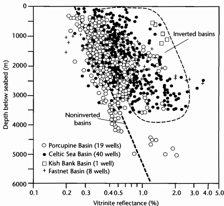
Fig. 9.35 Vitritine reflectance versus depth for Mesozoic and Cenozoic successions penetrated in boreholes in a number of basins offshore Ireland (Corcoran and Clayton 2001). Basins such as the Porcupine Basin show a “normal” R_o profile indicative of continual subsidence, whereas those basins that have experienced tectonic uplift and exhumation (such as the Celtic Sea, Kish Bank, and Fastnet Basins) have displaced R_o profiles indicating higher thermal maturity than expected from the present depth of burial.
