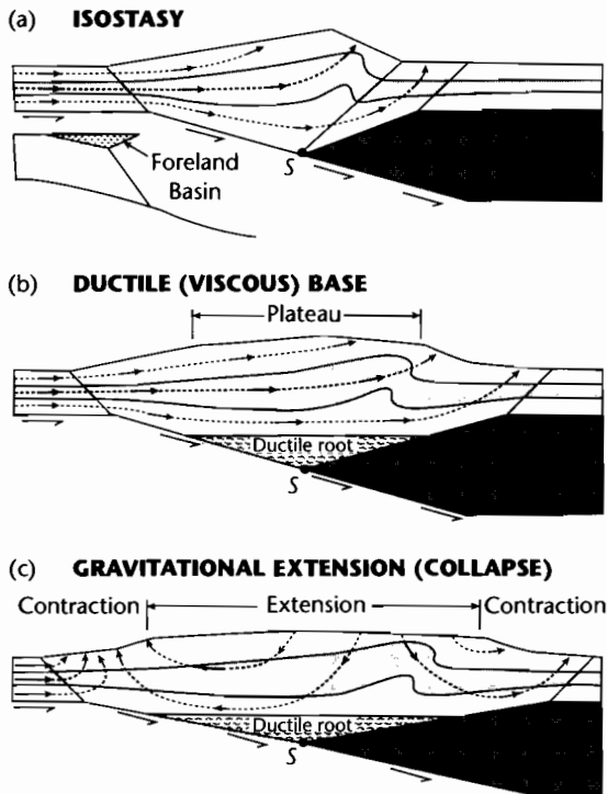
Fig. 4.28 The effects of isostasy and viscous (ductile) flow in the lower crust beneath a bivergent wedge (after Willett et al. 1993). In (a), isostasy causes the formation of flexural depressions (foreland basins); (b) Thickening of the bivergent wedge and increase in temperature decreases basal strength of the wedge and produces a ductile root. This promotes a reduction of surface slopes, resulting in a broad plateau. In (c), a further increase in lower crustal temperatures, or a decrease in the convergence rate causes the plateau to extend and increases contractional deformation in the bounding pro- and retro-wedges. Reproduced courtesy of Geological Society of America.
