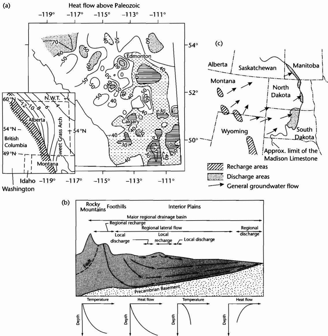
Fig. 9.18 Effects of groundwater flow on surface heat flows in sedimentary basins. (a) Heat flow map of southern and central Alberta, Canada based on estimated heat flow values (in \text{mW m}^{-2} ) above the top of the Paleozoic, based on 33,653 bottom hole temperature data from 18,711 wells (Majorowicz et al. 1984). The heat flows are strongly influenced by groundwater flow from recharge areas in structurally high regions, such as the Sweet Grass Arch (inset), to discharge areas; (b) Pattern of recharge and discharge in a cross-section from the Rocky Mountains to the Great Plains (after Majorowicz et al. 1984), and (c) plan view of groundwater flow in the Mississippian (Lower Carboniferous) Madison Limestone aquifer (after Downey 1984).
