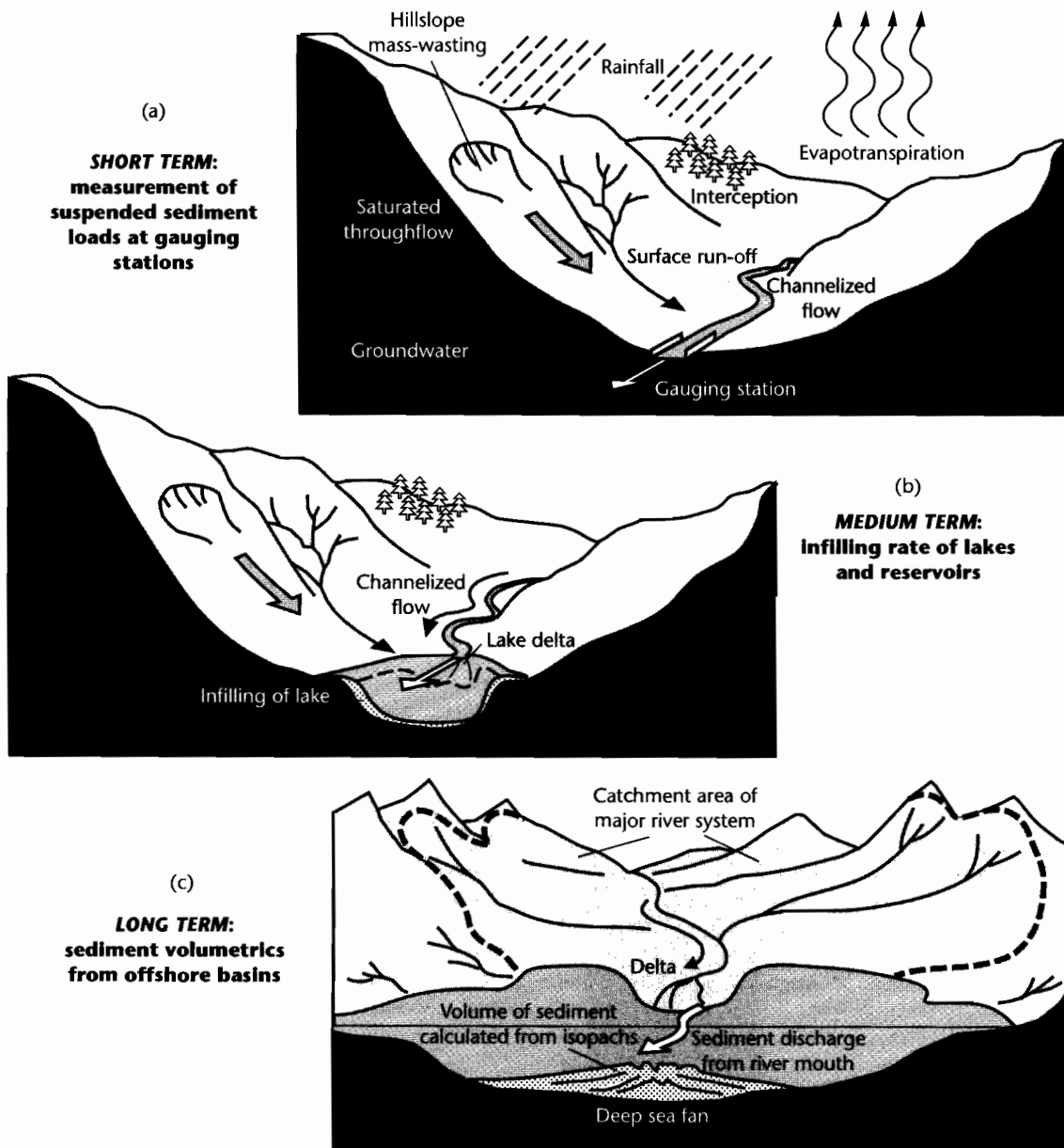
Fig. 7.4 Methods of estimating sediment yield. In (a), the short-term sediment yield is the discharge of sediment in \text{kg yr}^{-1} measured at a gauging station divided by the contributing catchment area. In (b), the medium-term sediment yield is the infill rate of a lake basin or artificial reservoir divided by the contributing catchment area. In (c), the long term sediment yield is the solid sediment volume derived from sediment isopachs of dated intervals of the stratigraphy divided by the paleocatchment area.
