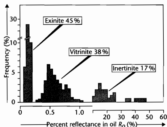
Fig. 10.21 Histograms showing reflectance measurements on different groups of kerogen particles. The exinite, vitritine, and inertinite groups each have different ranges of reflectance. The reflectance of vitritine is used as an index of thermal maturity (Ch. 9). Middle Liassic shale, Luxembourg, modified by Tissot and Welte (1978) from Hagemann (1974).
