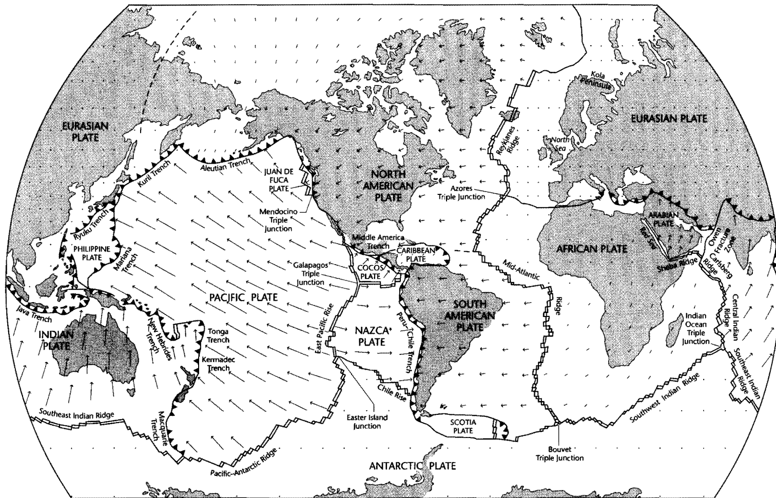
Fig. 1.5 The lithospheric plates, showing mid-ocean ridges, trenches, and transform boundaries (Le Pichon et al. 1973) and absolute motion vectors from Minster and Jordan (1978). Length of arrows is proportional to the plate speed. The fastest plate motion is in the western Pacific and Indian Oceans, whereas Africa, Antarctica, and Eurasia are almost stationary with respect to the mantle reference frame. Reproduced courtesy of American Geophysical Union.
