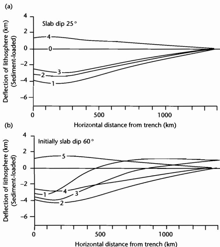
Fig. 5.11 Dynamic topography profiles generated by a model involving block subduction, with \Delta T = -700 K, D = 10^{24} Nm, for slab dips of 25^\circ (a) and initially 60^\circ (b). (a) The sequence of profiles shows the maximum dynamic subsidence (1), then profiles 10 Myr (2) and 25 Myr (3) after the cessation of subduction. Assuming the dynamic subsidence is filled with sedimentary rocks (density 2300 \text{ kg m}^{-3} ), the surface potentially (no erosion) rebounds to profile (4); (b) Sequence of profiles shows the dynamic topography as the subduction geometry changes from 60^\circ (1) to 25^\circ (2) and back to 60^\circ (3). The deflection 25 Myr after the cessation of subsidence is shown in (4), while the surface of the sedimentary basin, assuming the maximum deflection is filled with sedimentary rocks and no erosion, is shown as (5). Modified from Mitrovica et al. (1989). Reproduced courtesy of American Geophysical Union.
