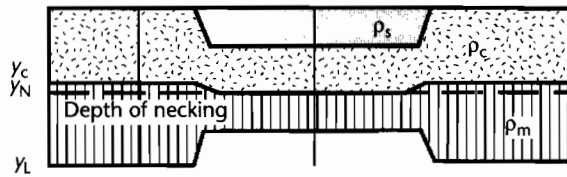
Fig. 3.28 Regional isostatic response to different depths of necking, based on Braun and Beaumont (1989), Kooi et al. (1992), Cloetingh et al. (1997). y_c , y_L , and y_N are the initial thicknesses of the crust and lithosphere and the necking depth respectively; \rho_c , \rho_m , and \rho_s are the densities of the crust, mantle, and sediments respectively. In (a) a shallow depth of necking results in a net downward acting force on the lithosphere, causing a regional downward flexure. In (b) the necking depth is deep, resulting in an upward acting force on the lithosphere that causes flexural uplift of the rift flanks.
