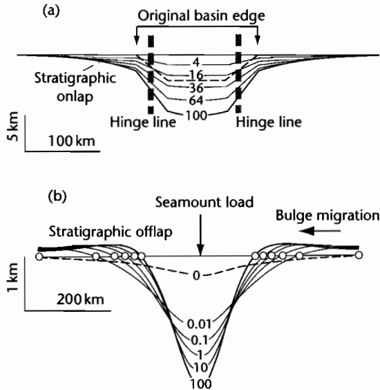
Fig. 8.15 Contrast of elastic and viscoelastic behaviors. (a) Stratigraphy of a model stretched basin with \beta = 2.0 , overlying an elastic lithosphere where the equivalent elastic thickness is the depth to the 450^{\circ}\text{C} isotherm. T_e increases with thermal age, causing stratigraphic onlap (steer's head geometry); (b) Response of a viscoelastic lithosphere with a viscous relaxation time of 10^4 yr to seamount loading. The lithosphere weakens rapidly following loading, causing stratigraphic offlap and a gradually narrowing basin. Vertical exaggeration of \times 10 . Numbers are time in Myr since rifting. After Watts et al. (1982).
