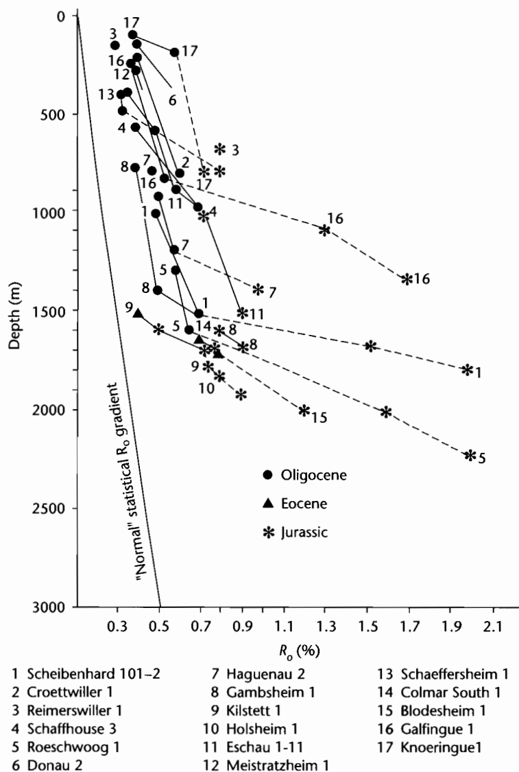
Fig. 9.33 Reflectance profiles from a number of wells in the Alsace region of the Rhine Graben (after Teichmüller 1970). In general, there are pronounced doglegs in the R_o profiles at about the age of the Oligocene–Eocene boundary. The post-Eocene history shows a “normal” gradient, whereas the pre-Oligocene sedimentary rocks have high reflectance values in relation to their depth of burial. This suggests that rifting in the late Eocene caused higher than normal maturity in the older rocks of the basin-fill.
