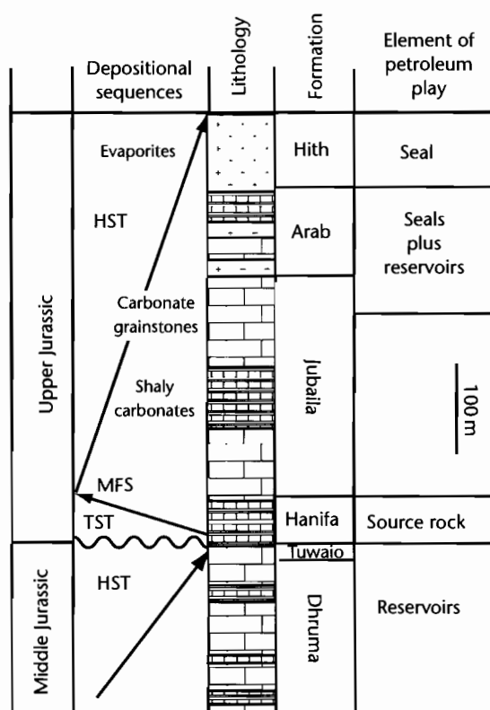
Fig. 10.37 Stratigraphic column of the Middle and Upper Jurassic of Saudi and the Persian Gulf, modified after Droste (1990). The Hith Formation constitutes an excellent regional topsal. Arab carbonate reservoirs are sealed by Arab evaporitic beds. The Hanifa Formation is an important source rock. Reproduced courtesy of Elsevier.
