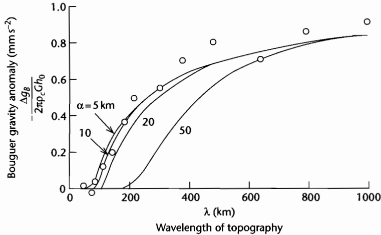
Fig. 2.29 Correlation of Bouguer gravity anomalies with topography (admittance) for the United States (Dorman and Lewis 1972), compared with the gravity formula for loading by periodic topography for different values of the flexural parameter \alpha = [4D/(\rho_m - \rho_s)g]^{1/4} in km. The best agreement is with \alpha \approx 20 km, or flexural rigidity D \approx 10^{21} Nm, which with E = 60 GPa and \nu = 0.25 , gives an equivalent elastic thickness T_e of 6 km. Reproduced courtesy of Cambridge University Press.
