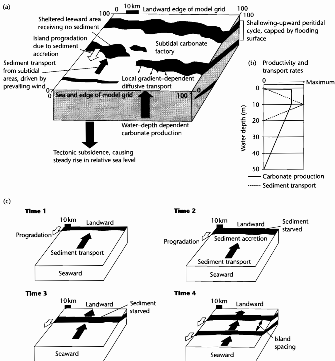
Fig. 8.32 Model for the generation of unforced high resolution cyclicity in peritidal carbonates, after Burgess et al. (2001). (a) Illustration of different processes involved in generating prograding inter- and supratidal islands and autocyclic shallowing-upward cycles; (b) Depth-dependent carbonate productivity relationship and sediment transport rate; (c) Different stages in the evolution of prograding islands. Time 1: landward transport of sediment causes accretion of inter- and supratidal flat. Time 2: Continued accretion drives inter- and supratidal flat progradation, which causes a sediment starved leeward side to develop. Time 3: Sediment starved lee subsides and prograding island forms, allowing a new subtidal carbonate factory to develop. Time 4: A second island system develops as the entire process is repeated. Reproduced courtesy of Blackwell Publishing Ltd.
