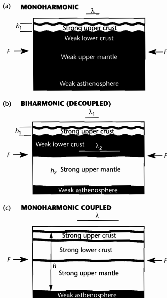
Fig. 4.19 Different styles of periodic buckling by a compressional force F ; h_1 and h_2 are the thicknesses of the competent crust and mantle respectively, which fold with wavelengths \lambda_1 and \lambda_2 . Where the lower crust is very weak, the upper crust and mantle lithosphere fold with different wavelengths ( \lambda_1 < \lambda_2 ), producing decoupled or biharmonic folding (b). Where there is a single coherent layer of coupled crust and mantle, as in both young (<150 Ma) and very old (>1000 Ma) lithospheres, monoharmonic folding develops (a) and (c). After Burov et al. (1993) and Cloetingh et al. (1999).
