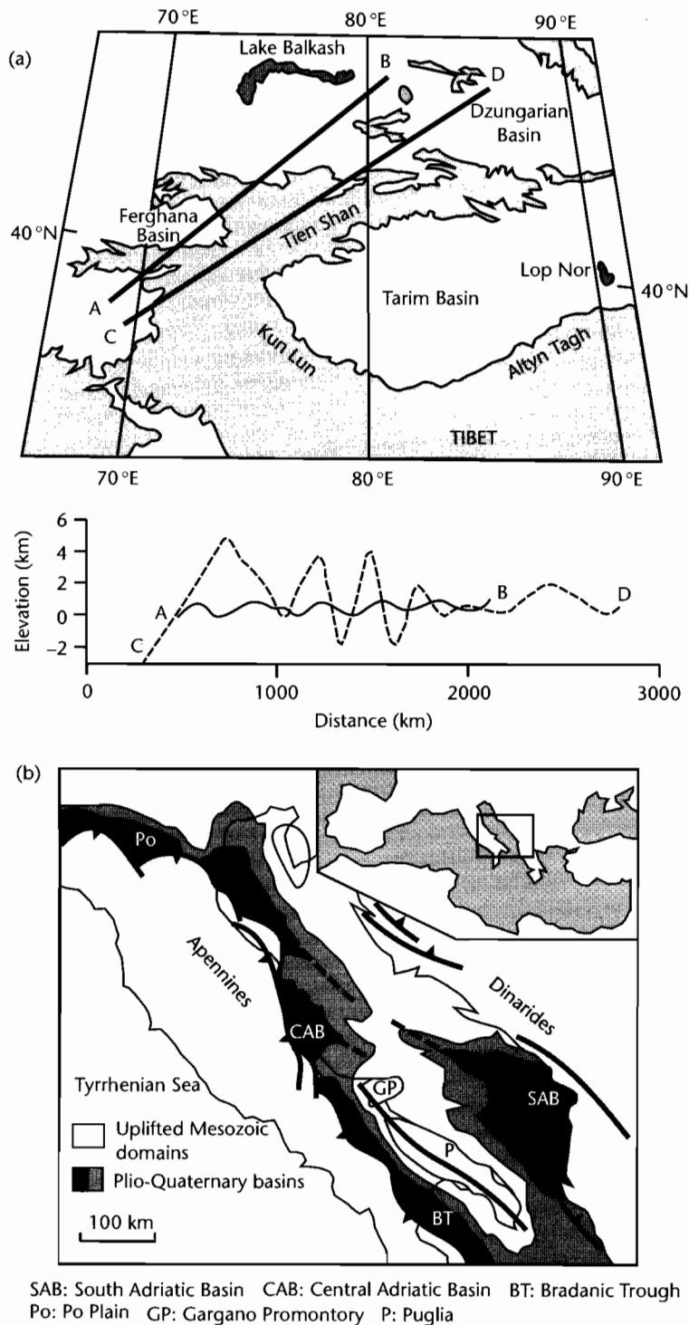
Fig. 4.20 Real-world examples of buckling from (a) central Asia (Cloetingh et al. 1999), showing elevation profiles for two transects A–B and C–D, and (b) Adriatic and eastern Italy (Bertotti et al. 2001), showing basins and highs oriented parallel to the strike of the Apennines and Dinarides. Reproduced courtesy of American Geophysical Union.
