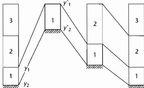
Fig. 9.6 Concept of the successive stages in a decompaction exercise.
