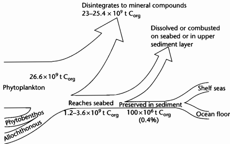
Fig. 10.7 Fate of the 26.6 \times 10^9 tons of annual organic carbon ( \text{C}_{\text{org}} ) production in the world's oceans. In the order of 0.4% is preserved in the bottom sediments of shelf seas and ocean floors.
