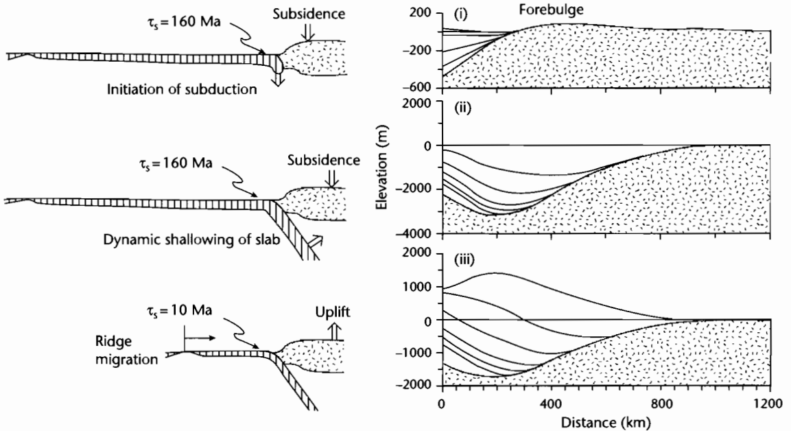
Fig. 5.12 Three stages in the evolution of dynamic topography over a subduction zone (a) and the associated chronostratigraphic surfaces in the region of the continental plate affected by dynamic topography (b). (i) An old (160 Ma) slab initially dips vertically, then penetrates the mantle by 100 km. The chronostratigraphic surfaces are separated by 2 Myr if the slab descent rate is 50 \text{ mm yr}^{-1} . The slab then shallows in dip (ii). Chronostratigraphic surfaces are shown for each 10^\circ decrease in slab dip. In (iii), the age of slab at ocean trench progressively decreases to 10 Ma, causing uplift (no erosion). After Gurnis (1992). Reproduced courtesy of American Association for the Advancement of Science.
