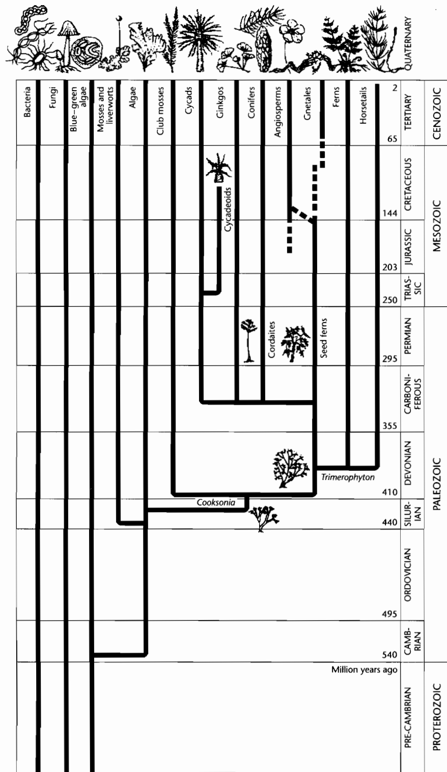
Fig. 10.10. Plant evolution over the last 600 Myr. The first land plants (primitive vascular varieties) such as Cooksonia appeared in the Silurian. A large number of new groups evolved in the Devonian. Important changes in land plant floras have taken place since the Silurian which have affected their hydrocarbon-generating characteristics. Only Mesozoic and Tertiary land plants have significant oil-generating potential. Today, two main groups dominate the land: the conifers , which cover over more than 10 \times 10^6 \text{ km}^2 of the Earth's surface, mainly in the cooler, drier areas, and flowering plants (angiosperms), which occur everywhere. The conifers may date back as far as the Carboniferous. The oldest definite flowering plants in the geological record are Barrenian (Early Cretaceous), but some authors place their origin in the Late Jurassic. In the sea, organisms adapted to life in water, such as the algae, have undergone their own evolution.
