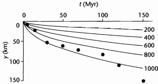
Fig. 2.17 Calculated isotherms for an oceanic lithosphere that is instantaneously cooled. The values of the isotherms are T - T_s °K. The dots are the estimated thicknesses of the oceanic lithosphere in the Pacific, from Leeds et al. (1974).
