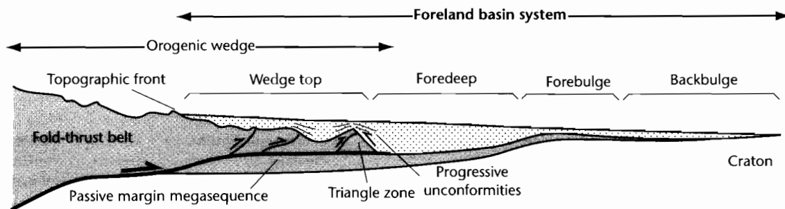
Fig. 8.57 The four depositional zones of a foreland basin system as envisaged by DeCelles and Giles (1996).
