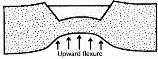
Fig. 3.28 Regional isostatic response to different depths of necking, based on Braun and Beaumont (1989), Kooi et al. (1992), Cloetingh et al. (1997). y_c , y_L , and y_N are the initial thicknesses of the crust and lithosphere and the necking depth respectively; \rho_c , \rho_m , and \rho_s are the densities of the crust, mantle, and sediments respectively. In (a) a shallow depth of necking results in a net downward acting force on the lithosphere, causing a regional downward flexure. In (b) the necking depth is deep, resulting in an upward acting force on the lithosphere that causes flexural uplift of the rift flanks.
