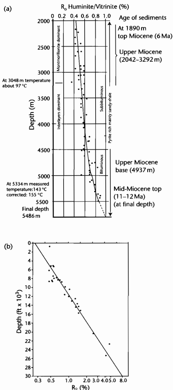
Fig. 9.32 (a) Vitritine reflectance profile for Terrebonne Parish, Pont au Fer well in Louisiana. The profile is sublinear and continuous, suggesting a near-constant geothermal gradient through time (after Heling and Teichmüller 1974); (b) Woodford Shale of the Anadarko Basin also shows a good sublinear trend (Cardott and Lambert 1985). Note logarithmic scale.
