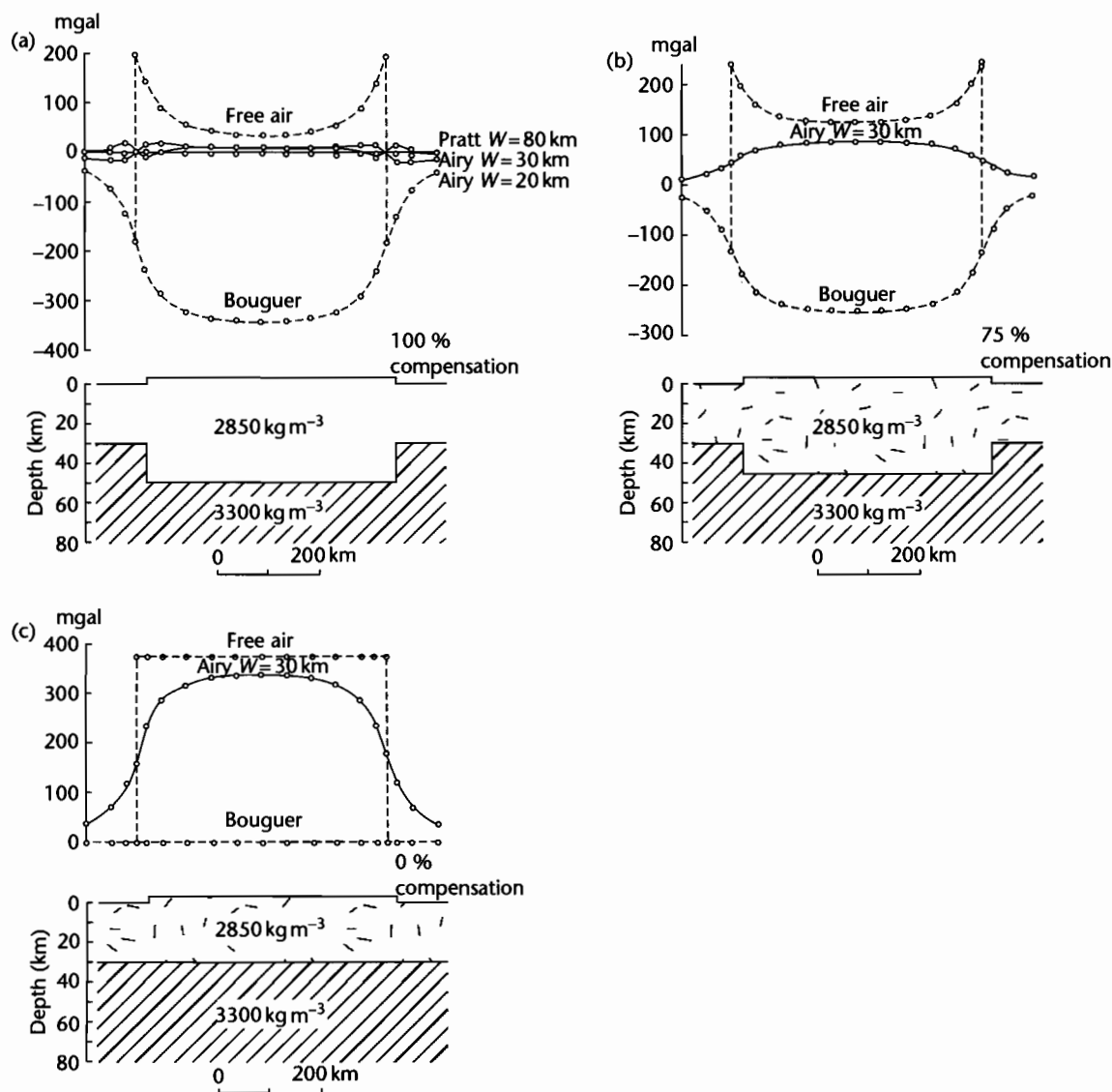
Fig. 2.28 Gravity anomalies over a schematic mountain range (Bott 1982 in Fowler 1990). In (a) the mountain range is 100% compensated (Airy isostasy); in (b) it is 75% compensated (Airy), and in (c) the mountain range is uncompensated. Solid lines: isostatic anomalies calculated for the different density models shown using Pratt compensation depth W=80 \text{ km} , Airy compensation depths W=20 \text{ km} and 30 \text{ km} . Dashed lines, free-air and Bouguer anomalies that would be measured over the mountain range. Reproduced courtesy of Elsevier.
