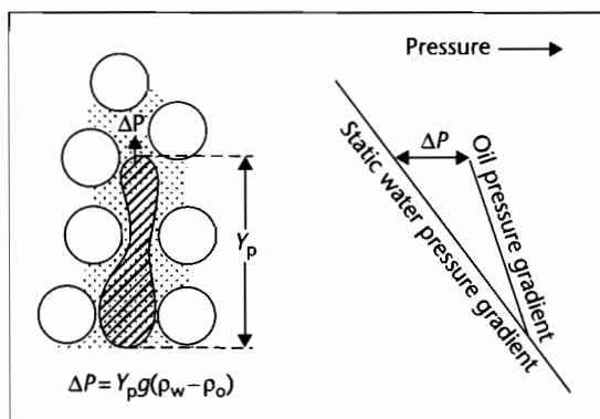
Fig. 10.30 Buoyancy as a driving force in secondary migration. Buoyancy is the pressure difference between a point in the petroleum column and the surrounding pore water. It is a function of the petroleum/water density difference and the height of the petroleum column. A large buoyancy pressure may develop at the tops of large, low-density (gas) petroleum columns. Pressure measurements at points throughout the petroleum column define a petroleum pressure gradient; this intersects the hydrostatic gradient at the petroleum–water contact.
