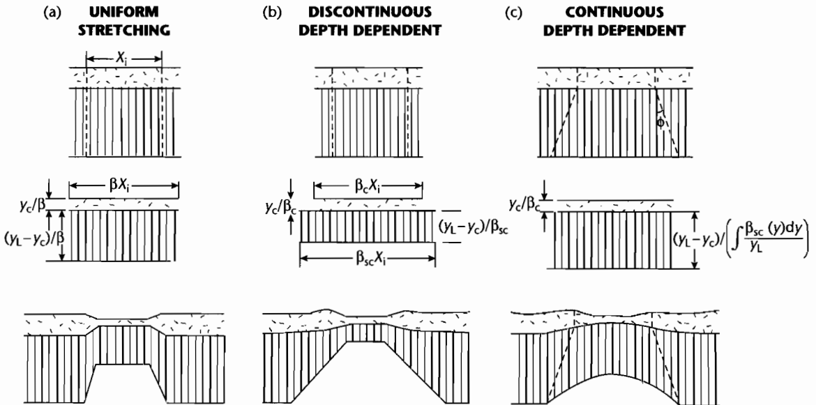
Fig. 3.18 Schematic diagrams to illustrate differences between (a) uniform, (b) discontinuous, and (c) continuous depth-dependent stretching. (a) Uniform extension in which the crust and subcrustal lithosphere extend by identical amounts; (b) Discontinuous depth-dependent extension in which the crust extends by a different amount to the subcrustal lithosphere, necessitating a decoupling between the two layers. The crustal and subcrustal extensions are independent but are uniform throughout the crust and subcrustal lithosphere (Royden and Keen 1980; Beaumont et al. 1982; Hellinger and Schlatter 1983); (c) Continuous depth-dependent extension in which the stretching is a continuous function of depth in the subcrustal lithosphere and the crustal stretching is the same as in (a) and (b) (Rowley and Sahagian 1986).
