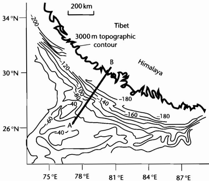
Fig. 4.4 The Himalaya and Ganga Basin. (a) Isopach map of sediment thicknesses in the Himalayan foreland basin, based on Raiverman et al. (1983); (b) Contours of Bouguer gravity anomaly over the Ganga Basin, and (c) observed Bouguer gravity anomalies along profile A-B, compared with the anomalies computed assuming the topography is locally compensated (Airy model) by thickening of the crust beneath central India. Note that there is an apparent mass excess in the Himalaya and a mass deficit over the Ganga Basin (after Lyon-Caen and Molnar 1985).
