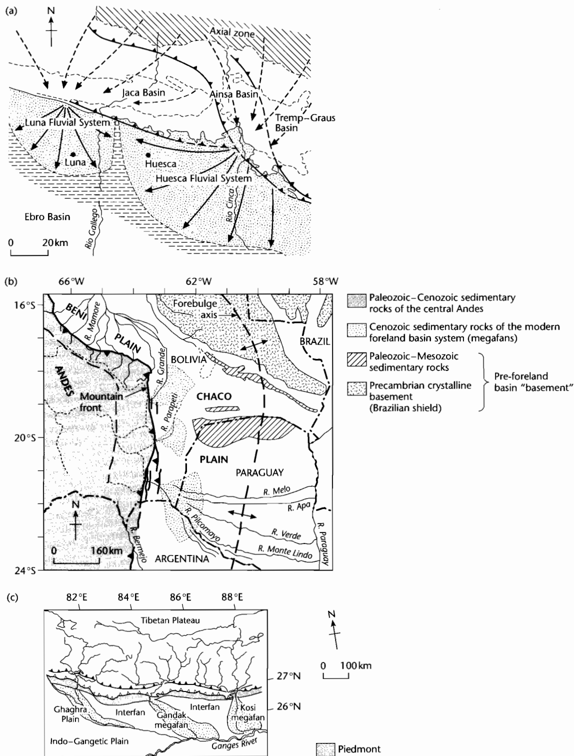
Fig. 8.59 Sediment dispersal patterns by rivers at mountain fronts. Large systems draining deep into the axial zones of orogenic belts break through the mountain front at re-entrants, producing large, low-gradient fans and megafans. Between the megafans are small, catchment–fan systems with local catchments. (a) Southern Pyrenees (Hirst and Nichols 1986), (b) Andes (Horton and DeCelles 1997), and (c) Himalayas (Gupta 1997). Note large variations in scale. (b), (c) Reproduced courtesy of Geological Society of America.
