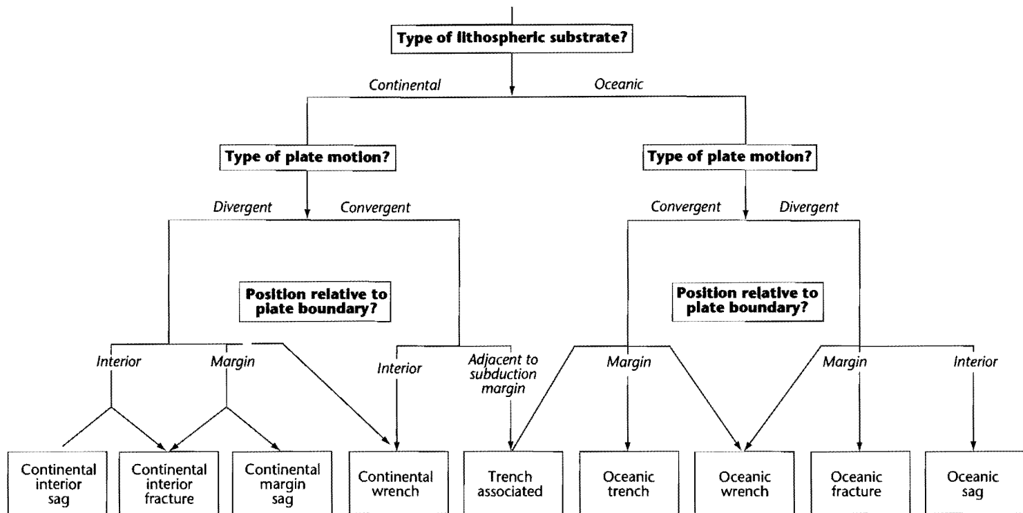
Fig. 1.10 Basin classification scheme based on Kingston et al. (1983a, b). Not all basin types appear in this scheme. Most notably, foreland basins are missing.
