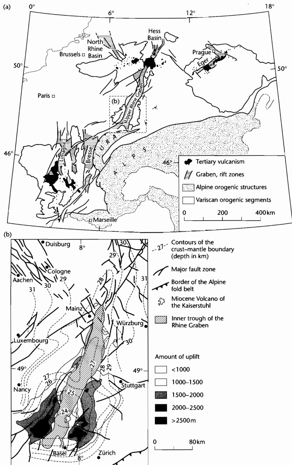
Fig. 3.3 (a) Location of main elements of the late Eocene–Recent Western European Rift System, with sites of Tertiary volcanicity; (b) Depth to the Moho below sea-level (in km), showing a mantle bulge in the southern Rhine Graben centred on the Kaiserstuhl volcano (Illies 1977). The largest amounts of denudation are found on the rift flanks above the shallow mantle. Reproduced courtesy of the Board of the Stichting Netherlands Journal of Geosciences.
