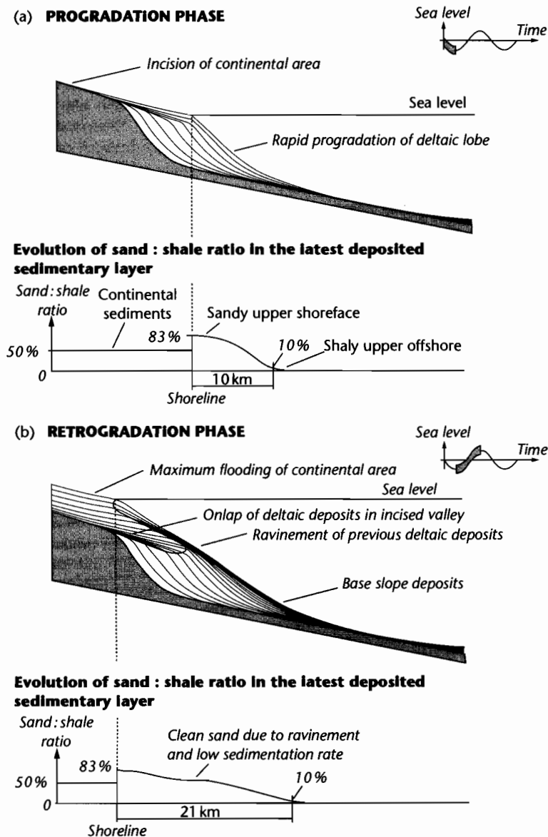
Fig. 8.36 Computer-generated 2-D transects through a fluvial-dominated delta, showing the sand:shale ratio in the preserved sediment during the progradational phase (a) and retrogradational stage (b). After Granjeon and Joseph (1999). Reproduced courtesy of Society for Sedimentary Geology.
