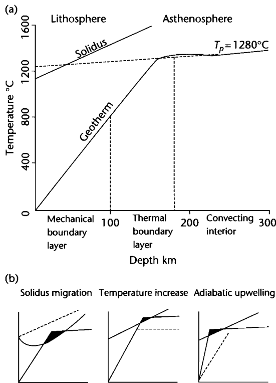
Fig. 3.39 Causes of partial melting related to lithospheric extension (after McKenzie and Bickle 1988, Latin et al. 1990, and Leeder 1995). (a) Geotherm for a potential temperature of 1280°C and solidus for mantle material. The potential temperature is the temperature on an adiabatic gradient extrapolated to surface pressure; (b) Adiabatic decompression may be facilitated by migration of the solidus caused by the presence of volatiles such as water, by a temperature increase due the presence of a plume in the asthenosphere, or by mechanical thinning of the lithosphere and asthenospheric upwelling.
