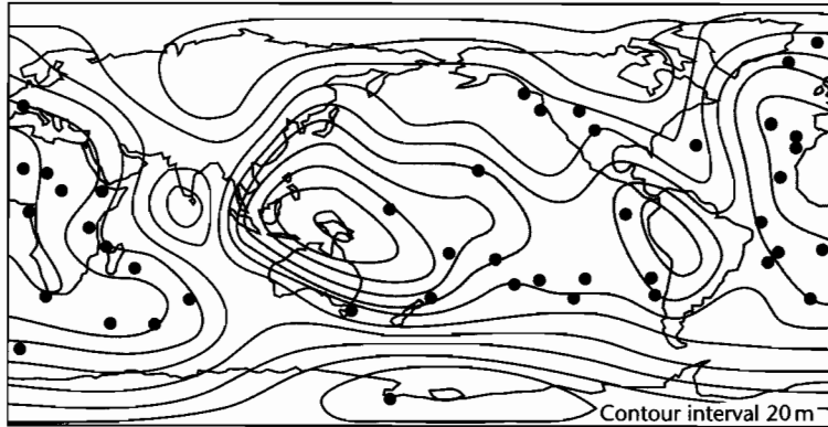
(b) Residual geoid: degree 2–10
