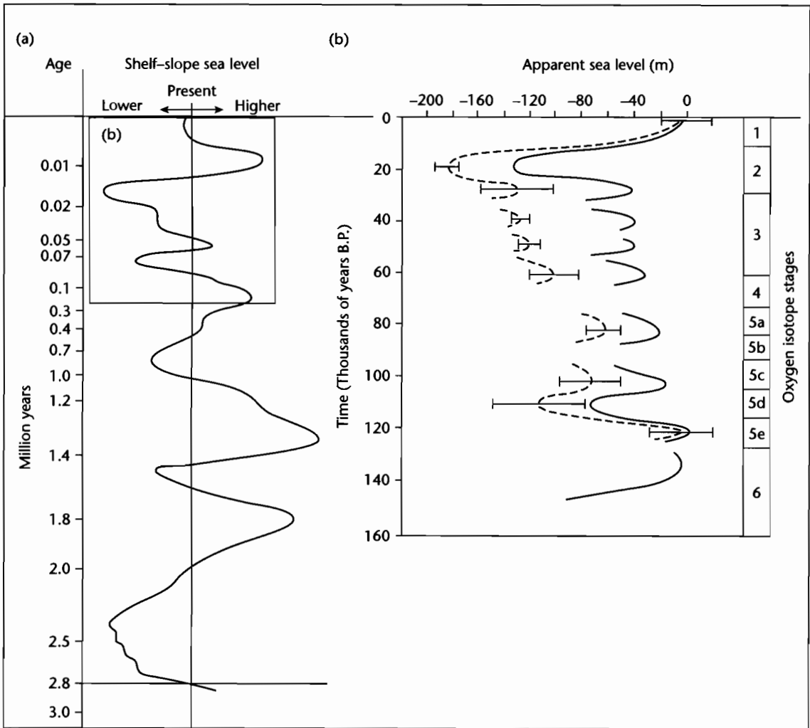
Fig. 8.31 (a) Inferred Pleistocene sea-level fluctuations in the northwestern Gulf of Mexico since 3 Ma (after Morton and Price 1987), derived by Smith (1965) from interpreted water depth and paleotemperatures, and modified by Beard et al. (1982). Note non-linear scale for age; (b) Detailed glacio-eustatic record (dashed line, Moore 1982) and oxygen isotope record based on deep sea benthic foraminifera (solid line, Williams 1984) for the last 130 000 yr (after Suter et al. 1987).
