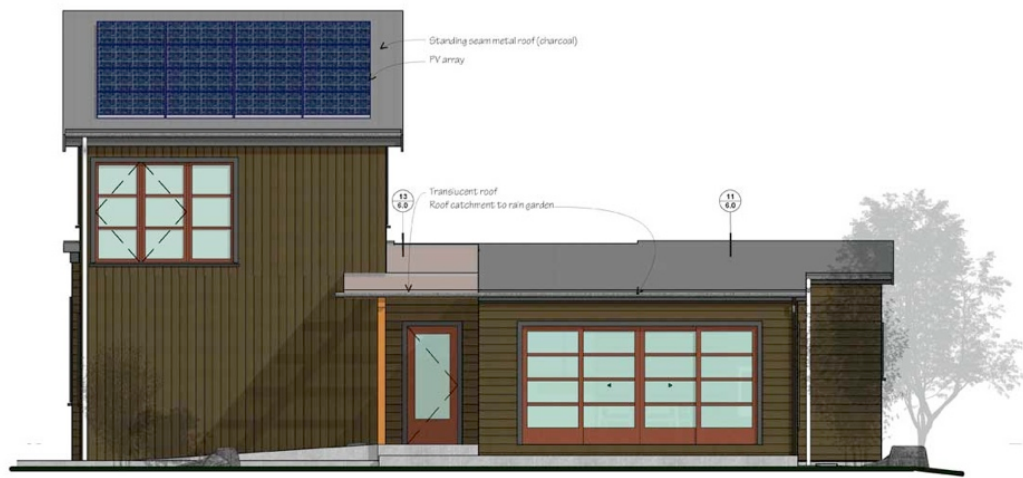
South Elevation 1/4" = 1'-0"
