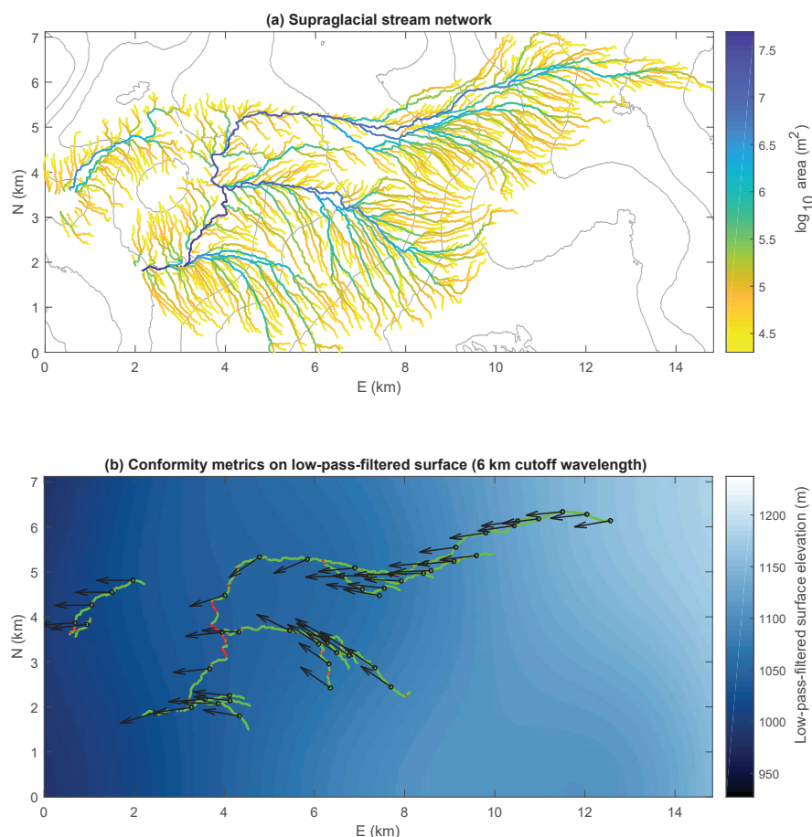
Figure 6. (a) Supraglacial stream network obtained by flow routing on 2 m DEMs from study region R1 (Fig. 1a, Table 1), colored by accumulated upstream drainage area. Surface elevation is shown with 20 m black contours. Fluvial incision rate should increase with increasing slope and drainage area (Eq. 7). (b) Illustration of stream conformity metrics for select streams from the same network, projected onto topography low-pass filtered at a 6 km cutoff wavelength. Sections of streams that would be flowing uphill on this filtered surface are colored red and other sections are green; these data are used to calculate percent downhill \%d . Black arrows indicate the steepest descent directions on this filtered surface; the angle between these directions and the corresponding stream channel orientations is used to calculate the conformity factor \Lambda .
