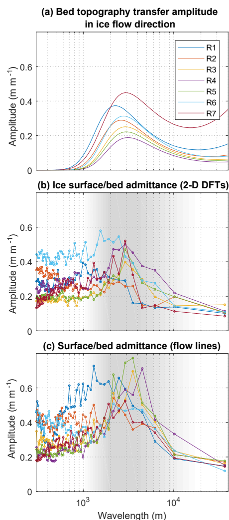
Figure 7. (a) Predicted bed topography transfer amplitudes from our seven study regions (Fig. 1a, Table 1), with \eta = 10^{14} Pa s and C^{0*} = 10 in all regions. (b) Results from one method for calculating empirical admittance of measured bed topography to observed ice surface topography by binning and averaging absolute wave number components of 2-D DFTs (see Sect. 2.3.5). (c) Results from a second method for calculating empirical bed-to-surface admittance by binning and averaging 1-D DFTs from multiple ice flow line transects. For all regions both calculations of empirical admittance (b, c) generally match predicted transfer amplitudes (a) at wavelengths greater than \sim 1 km and exhibit similar peaks between \sim 1 and 10 km (shaded regions in b and c). At wavelengths less than \sim 1 km both empirical admittance calculations are higher than predicted transfer amplitudes.
