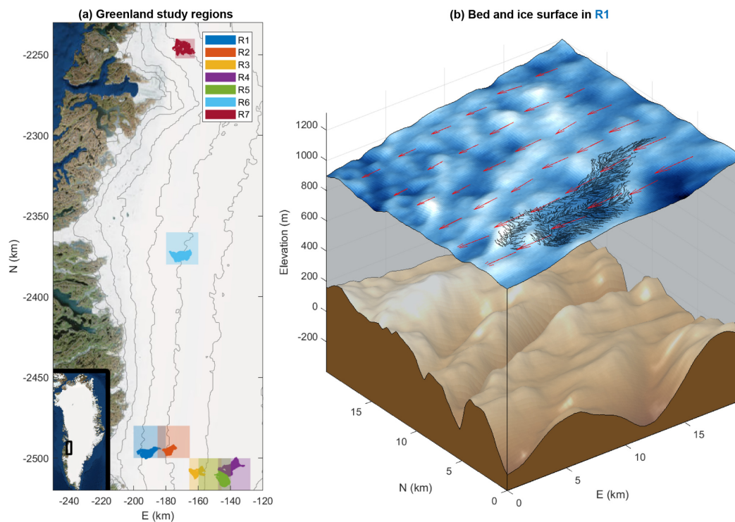
Figure 1. (a) Study IDCs (solid colored patches) of western Greenland with bounding boxes (semitransparent squares) indicating the corresponding domain used for bed transfer and admittance calculations. Black 200 m elevation contours are from BedMachine/GIMP (Howat et al., 2014; Morlighem et al., 2017a). Imagery is from the ArcGIS ERSI world imagery base map. Information on all regions is shown in Table 1. (b) Ice surface and bed elevations (from BedMachine/GIMP) in study region R1, with stream channels from the study drainage network shown in black and the velocity field shown by red arrows.
