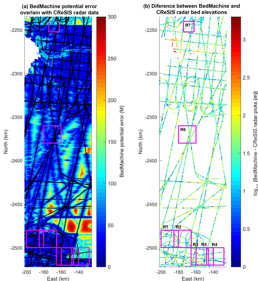
Figure 2. (a) BedMachine v3 potential bed elevation error overlain by CReSIS radar bed elevation picks (Morlighem et al., 2017a, b; CReSIS, 2016). BedMachine includes radar data from other sources not shown here and is also constrained with mass conservation modeling over most of the region shown. BedMachine error generally decreases where elevations are better constrained by radar data. Our study regions (magenta) encompass a broad range of bed DEM quality (Fig. 1a, Table 1). (b) Difference between bed elevations from BedMachine and CReSIS radar picks (only including radar picks marked as good quality). In many regions there is appreciable scatter in radar elevation picks and significant error in the derived bed DEM; we examine the impact this uncertainty has on ice surface predictions.
