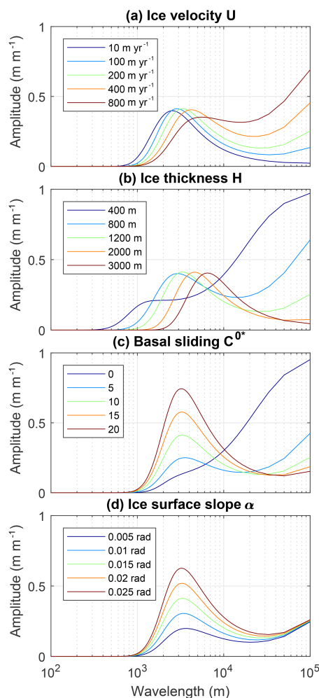
Figure 3. (a–d) Bed topography transfer function amplitudes in the ice flow direction (along an ice flow line). In all plots the parameters not otherwise indicated are U = 200 \text{ m yr}^{-1} , H = 1200 \text{ m} , C^{0*} = 0 , \alpha = 0.015 \text{ radians} , and \eta = 10^{14} \text{ Pa s} . The spread of plotted parameters broadly encompasses the range of parameters found in our study regions (Fig. 1a, Table 1). Transfer amplitude peaks between around 1 and 10 km for a wide range of parameters.
