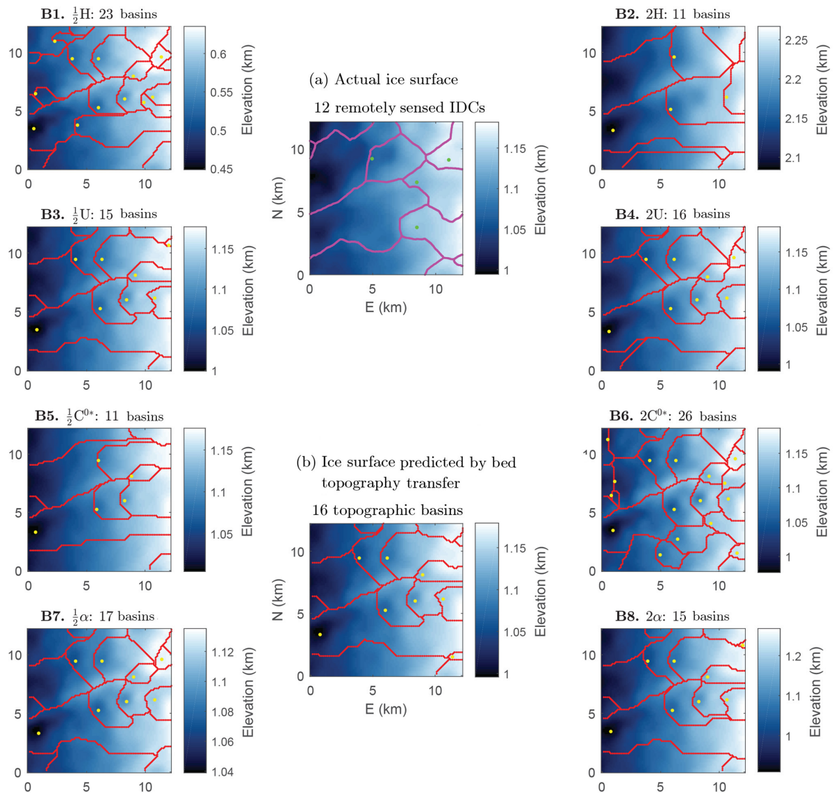
Figure 11. (a) IDCs (magenta outlines) and moulin (green dots) obtained from satellite images by Yang and Smith (2016). (b, B1–B8) Ice surface topographic basins (red outlines) and local minima (yellow dots) on ice surfaces predicted with bed topography transfer with various ice flow parameters. Study region R1 (Fig. 1a, Table 1) with \eta = 10^{14} Pa s and baseline C^{0*} = 10 . While the bed-transfer-predicted topographic basin configuration in (b) is different from the IDC configuration in (a), the basin densities are similar. Changing ice thickness H or basal sliding parameter C^{0*} by a factor of 2 produces significant changes in predicted topographic basin configurations (B1, B2 and B5, B6).
