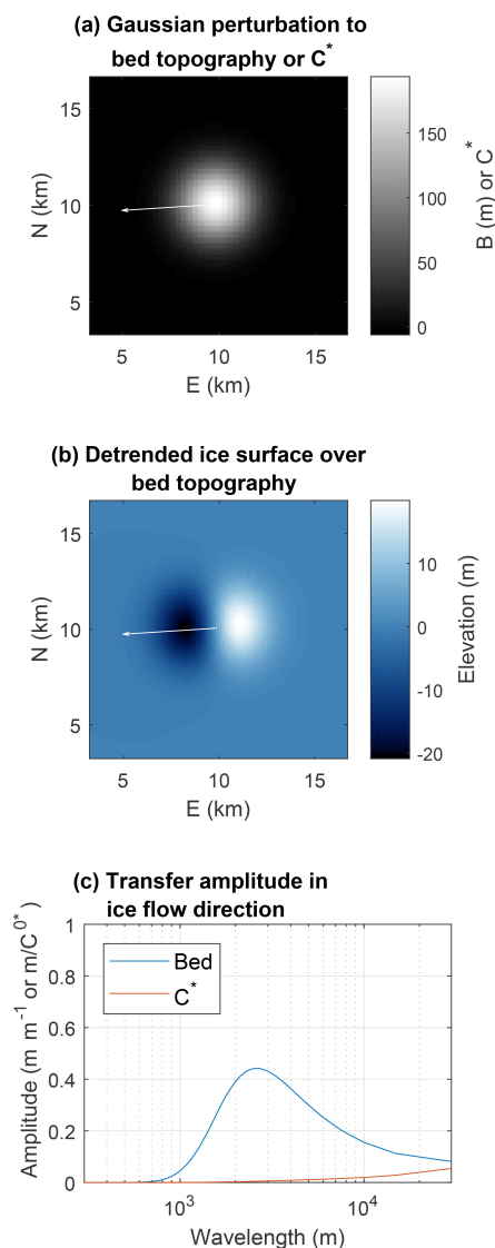
Figure 4. Illustration of steady-state basal transfer for ice flow parameters representative of the western Greenland ablation zone. Ice flow parameters are from region R1 (Fig. 1a, Table 1) with \eta = 10^{14} \text{ Pa s} . (a) Gaussian bed topography or basal sliding perturbation. (b) Detrended predicted ice surface over the Gaussian bed topography perturbation (with C^{0*} = 10 ). White arrows in (a) and (b) indicate the ice flow direction. (c) Transfer amplitudes in the ice flow direction (along a flow line) for bed topography and basal sliding C^{0*} perturbations. The transfer functions also have important phase components not shown here (see Gudmundsson, 2003). With these flow parameters, surface topography created from basal sliding perturbations should generally be of much lower amplitude than surface topography created from bed topography.
