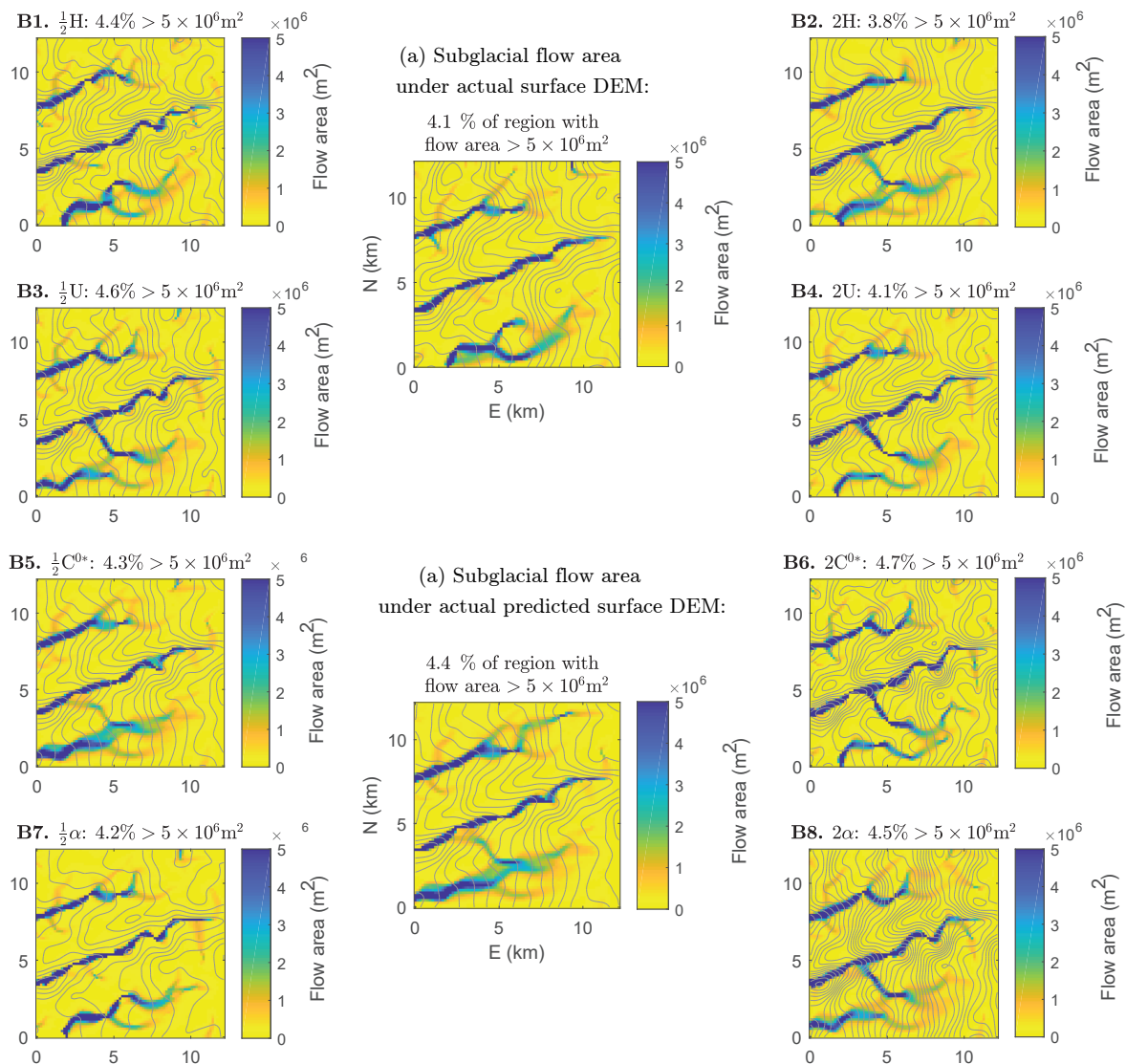
Figure 12. (a) Subglacial accumulated flow (drainage) area obtained via flow routing on hydraulic potential fields calculated under the actual ice surface DEM from BedMachine/GIMP (Howat et al., 2014; Morlighem et al., 2017a). Grey contours in all plots are 0.1 MPa hydraulic potential contours. (b, B1–B8) Subglacial accumulated flow area calculated under the ice surface predicted with bed topography transfer with various ice flow parameters. Study region R1 (Fig. 1a, Table 1) with \eta = 10^{14} Pa s and baseline C^{0*} = 10 . The flow area threshold displayed ( 5 \times 10^6 m 2 ) was chosen to highlight pathways of high relative water flux.
