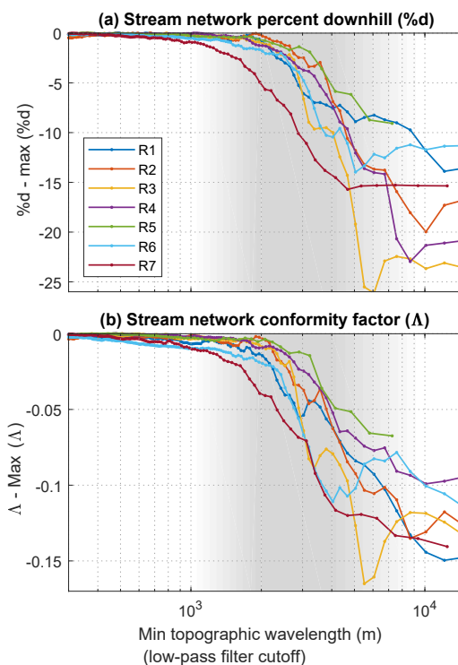
Figure 10. (a) Percent downhill \%d . (b) Conformity factor \Lambda . Values for both stream metric topographic conformity metrics are calculated in our seven study regions (Fig. 1a, Table 1). All values are normalized to the maximum values in each network due to the variability in plateau values of \%d and \Lambda among networks. For all supraglacial stream networks the cutoff filter wavelengths over which \%d and \Lambda decrease most significantly are between \sim 1 and 10 km (shaded regions), similar to the bed topography wavelengths predicted to transfer most strongly (Fig. 7).
