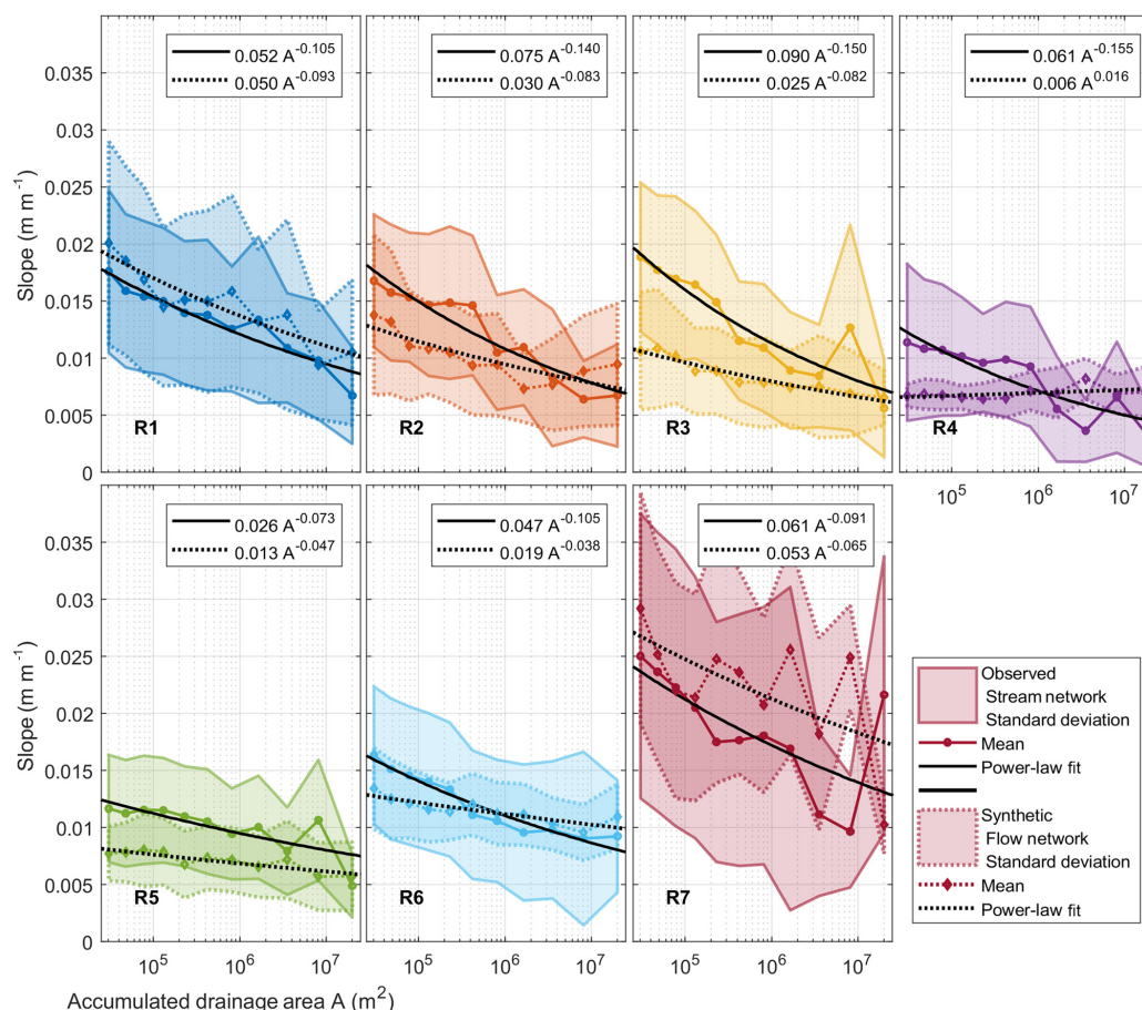
Figure 9. Mean stream channel slopes binned by accumulated upstream drainage–flow area from our seven study regions (Fig. 1a, Table 1). Results are shown from both observed supraglacial stream networks and synthetic flow networks calculated on surfaces predicted with bed topography transfer (see Sect. 2.4.2 and 2.4.3). The standard deviation of slope within each area bin is indicated by shaded patches, where patches with solid outlines correspond to observed stream networks and patches with dotted outlines to synthetic flow networks. Mean slopes are shown by solid and dotted colored lines and power-law fits by solid and dotted black lines. Under the (likely inaccurate) assumptions that supraglacial stream longitudinal elevation profiles are incisionally controlled and in a steady-state configuration under ice flow conditions analogous to uniform uplift, the power-law fit coefficients and exponents should correspond to K^{-1} and -m from Eq. (7). Synthetic flow networks from regions R3 to R5 and R6 may not be meaningful due to surface underprediction (see Sect. 3.2).
