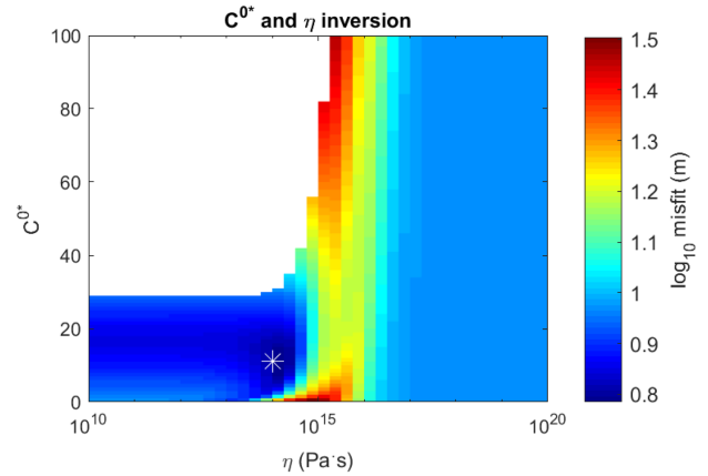
Figure 5. Misfit minimization for \eta and C^{0*} between the ice surface DEM and ice surfaces predicted by bed topography transfer in study region R1 (Fig. 1a, Table 1). The white star indicates the location of minimum misfit, at C^{0*} = 10 and \eta = 10^{14} . The blank plot area is the region where parameters are nonphysical (resulting in transfer amplitudes > 1 ).
