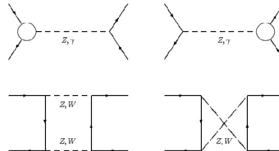
vertex corrections and box diagrams ( direct corrections )
