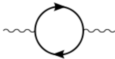
vacuum polarizations ( oblique corrections )
