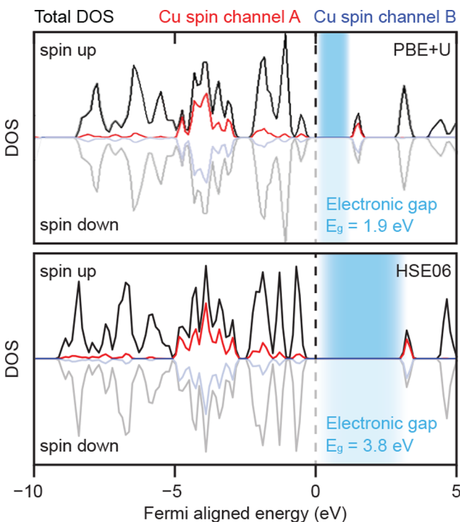
Figure 6. Comparison of density of states (DOS) of HKUST-1 obtained with DFT + U and HSE06. Both functionals produced similar DOS, however, hybrid/HSE06 yielded a larger band gap than DFT + U . Adapted with permission from ref 206. Copyright 2015 AIP Publishing.
