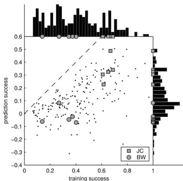
Figure 6. Summary of training and prediction success. Each point in the main panel represents the success of the STRF model in estimating the response to an individual stimulus (15 sec). For the training success (x-axis), the same individual stimulus was used for both estimating and testing the STRF. For the prediction success (y-axis), the STRF was tested on the individual stimulus but trained on all others. To permit the individual points on the graph to be resolved, only a subset of the stimuli ( n = 10 ; chosen randomly for each neuron) is shown. Although the prediction success provides a lower bound on the capability of the model to estimate the response, the training success yields an upper bound. Surprisingly, some of the stimuli are consistently better than others across neurons [compare JC (squares) and BW (circles)]. Hence, the STRF is able to capture a significant part of the response to some stimuli, yet it fails to predict the response to others. The distribution of training and prediction success is displayed as a histogram on the top and the right, respectively. Averaged over all stimuli and cells, the training success was 39%, and the prediction success was 11%. Hence, the responses of cortical neurons to natural stimuli are dominated by nonlinearities.
