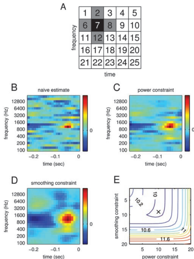
Figure 4. STRF estimation. To estimate a relationship between stimulus and response, we computed the STRFs of the recorded neurons. To circumvent estimation problems deriving from the usage of natural stimuli, we subjected the STRF estimation to a smoothing and power constraint. A , Range of smoothing constraints. The smoothing constraint enforces that the values of neighboring bins do not deviate too strongly. The neighbors of bin 7, for example, are shown in gray. B , Naive estimate of the STRF via linear regression. An estimate without any constraints achieves a mean square error \varepsilon = 5.6 \text{ mV}^2 between actual and predicted response on the data used for the STRF estimation (training) and an error \varepsilon = 10.69 \text{ mV}^2 on new data (prediction). The large difference indicates strong overfitting, which is also visible in the noisy structure of the STRF. C , Optimal estimate of the STRF subject to a power constraint. Here, the power constraint was chosen to minimize the prediction error. Indeed, whereas the training error increases ( \varepsilon = 6.95 \text{ mV}^2 ), the prediction error is now considerably lower ( \varepsilon = 9.97 \text{ mV}^2 ). D , Optimal estimate of the STRF subject to smoothing constraint. Both training error ( \varepsilon = 7.08 \text{ mV}^2 ) and prediction error ( \varepsilon = 10.01 \text{ mV}^2 ) are similar to those for the power constraint. E , Prediction error for different combinations of smoothing and power constraints. For this cell, combining the two types of constraints does not significantly enhance the prediction success. The absolute minimum ( \varepsilon = 9.97 \text{ mV}^2 ) is denoted by the black cross. The STRFs inside the trough (blue contours) are therefore equally valid estimates; showing the “extremes” in C and D allows an assessment of the robustness of the estimates.
